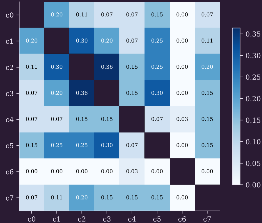
Hub Jaccard (top-15) (max off-diag = 0.36)
