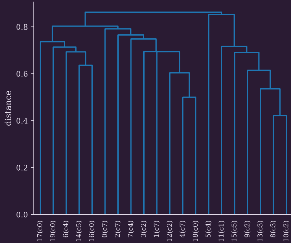
Hub Jaccard -- avg linkage
