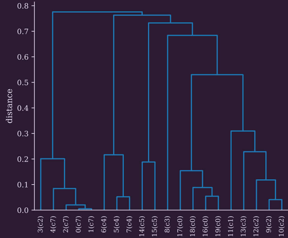
Composition cosine -- avg linkage
