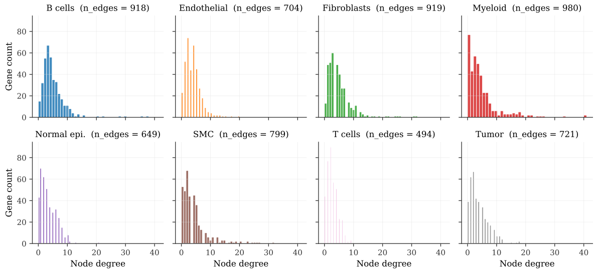
Figure 15: Degree distributions of the eight per-class GGMs at \alpha = 0.07 on the 378 common genes. All distributions are right-skewed (a small number of hubs concentrate connectivity), but tail length varies markedly across classes. T cells (Class 6) have the sparsest network ( n_{\text{edges}} = 494 , shortest tail), consistent with their dispersed, infiltrating spatial distribution; Myeloid cells (Class 3) have the densest ( n_{\text{edges}} = 980 , longest tail).
