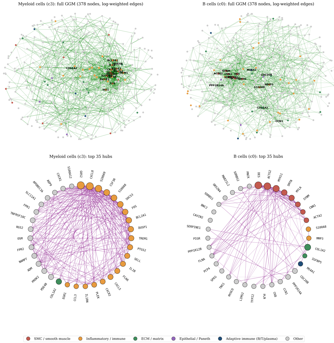
Figure 16: Gene networks of two contrasting cell-type classes: Myeloid cells (Class 3, left) and B cells (Class 0, right). Top row: full GGM on the 378 common genes, drawn as a force-directed network. Edge thickness and opacity are log-scaled by |\Theta_{ij}| , so the strongest conditional dependencies emerge from the cloud of weaker edges. Nodes are coloured by gene family (see legend); the top 15 hubs by degree are labelled. Bottom row: the same network reduced to its top 35 hubs by degree, displayed as a chord diagram sorted by family. The Myeloid network is dominated by inflammatory hubs (orange) that reinforce both cell-intrinsic identity and neighbourhood signal; the B-cell network is dominated by SMC markers (red), with MS4A1 (the only canonical B-cell hub) appearing as a single isolated blue node, consistent with diffusion of mRNA from spatially adjacent smooth muscle cells in perivascular tertiary-lymphoid microenvironments.
