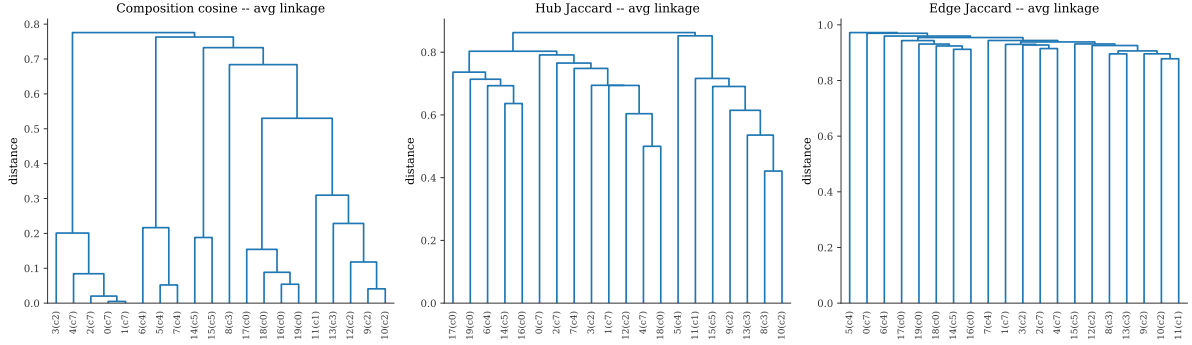
Figure 19: Hierarchical clustering of the 20 niches under three similarity measures, with average linkage. The composition dendrogram (left) is deep and cleanly grouped: same-dominant-class niches merge below 0.30, while the root sits at 0.776. The hub dendrogram (middle) is compressed into 0.42–0.86 and shows only weak family-level structure. The edge dendrogram (right) is nearly flat, with every merge between 0.878 and 0.972: in edge space, almost all niches are equally distant from each other.
