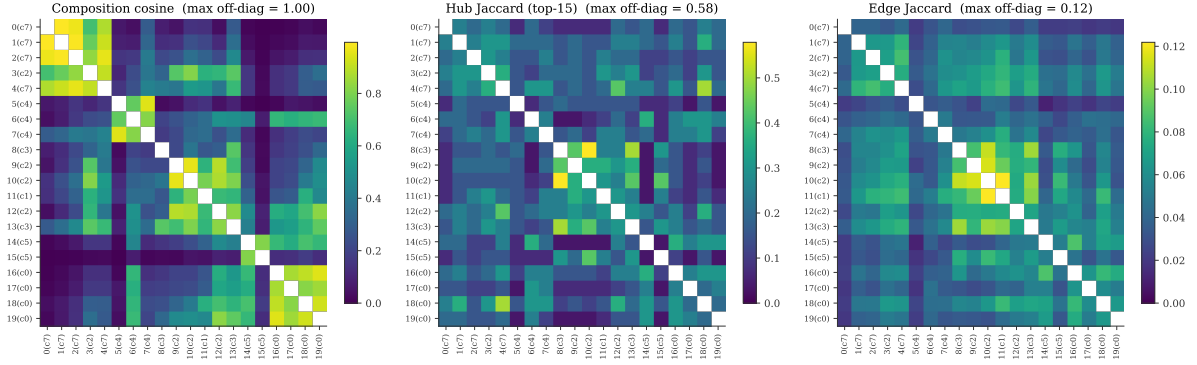
Figure 18: Pairwise similarity between the 20 per-niche networks under three measures: composition cosine (left, max off-diagonal 0.995), top-15 hub Jaccard (middle, max 0.58), and edge Jaccard (right, max off-diagonal 0.12). Diagonals are masked. Niches labelled by id and dominant class. The composition heatmap shows strong block structure (c7-niches in the upper-left, c0-niches in the lower-right). The hub heatmap shows weaker but visible block structure. The edge heatmap shows almost no block structure: niches share hubs much more than they share specific edges.
