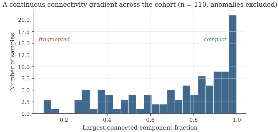
Figure 3: Histogram of the largest connected component fraction (LCF) across 110 samples (anomalies excluded). The distribution is left-skewed with a single mode near 1.0 and a long tail reaching 0.11; a Hartigan dip test finds no evidence of bimodality ( p = 0.93 ). The compact ( \text{LCF} \geq 0.90 , n = 37 ) and fragmented ( \text{LCF} \in [0.25, 0.45] , n = 19 ) labels used throughout the report are coarse summaries of the two ends of a continuum, not distinct architectures.
