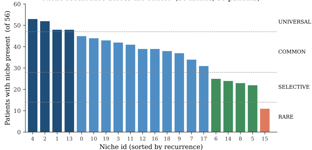
Niche recurrence across the cohort (20 niches, 56 patients)
