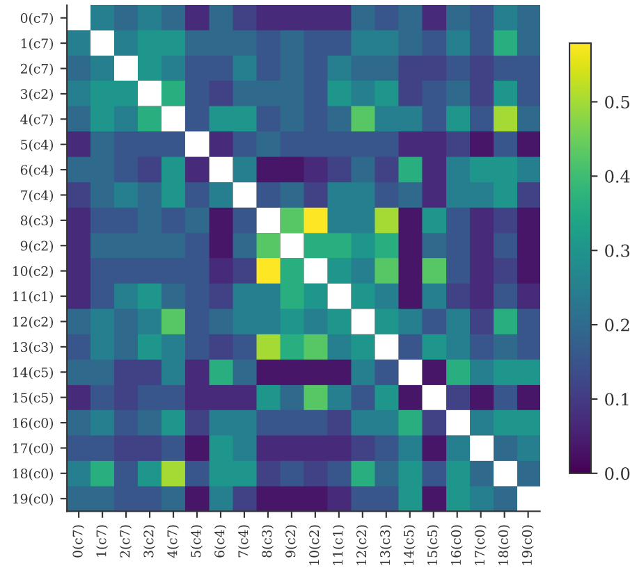
Hub Jaccard (top-15) (max off-diag = 0.58)
