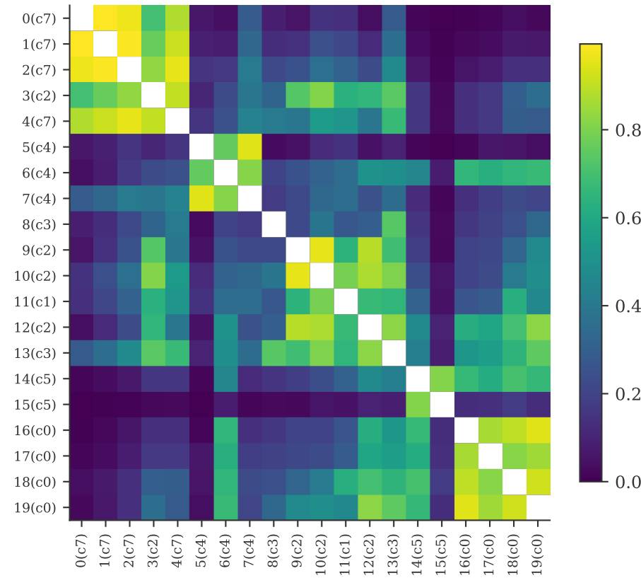
Composition cosine (max off-diag = 1.00)
