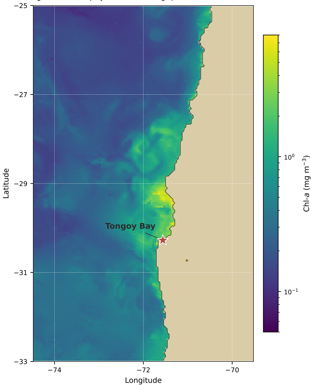
Regional chlorophyll (CMEMS L4 gap-free) --- 2025-12-20
