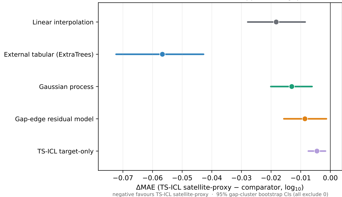
B. Paired MAE difference on matched support (449 gaps)
