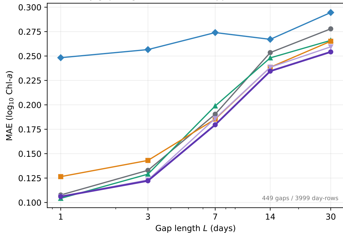
A. Error by gap length on matched support
