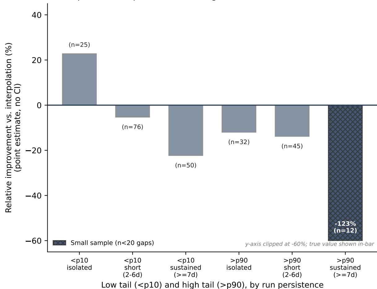
B. Tail-persistence performance (diagnostic)
