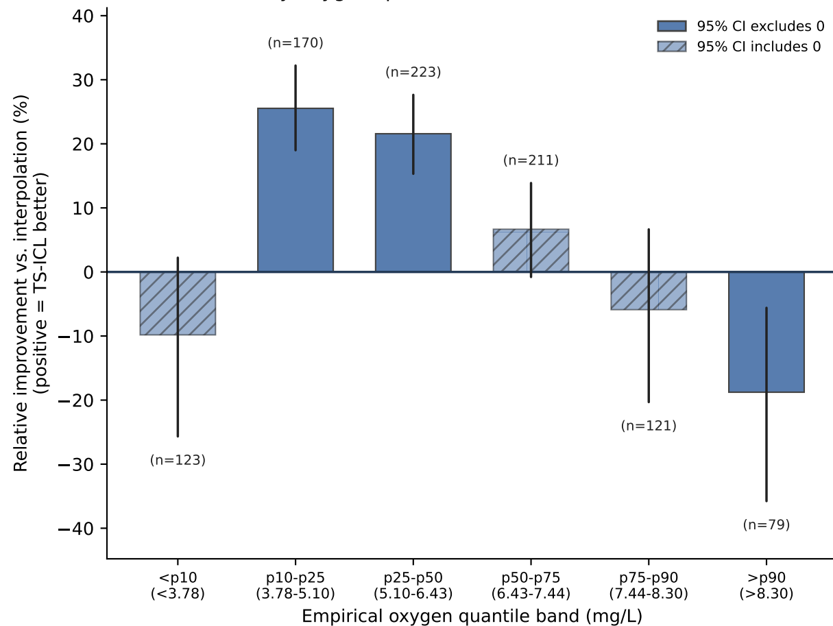
A. Performance by oxygen quantile band
