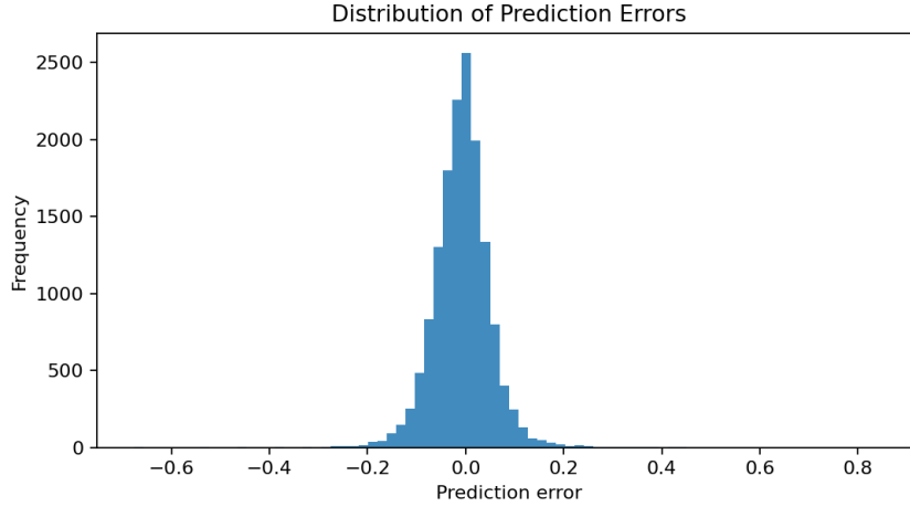
Figure 7.6: Distribution of neural network prediction errors.
