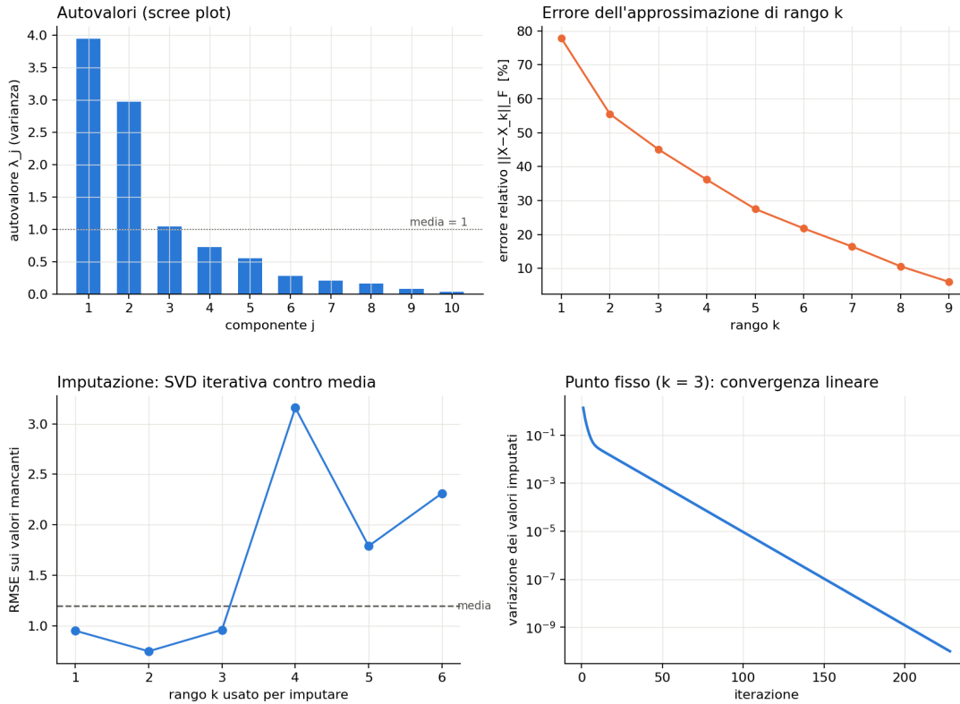
Figure 3: Top: eigenvalues and rank- k error. Bottom: imputation with iterative SVD and convergence of the fixed point.
