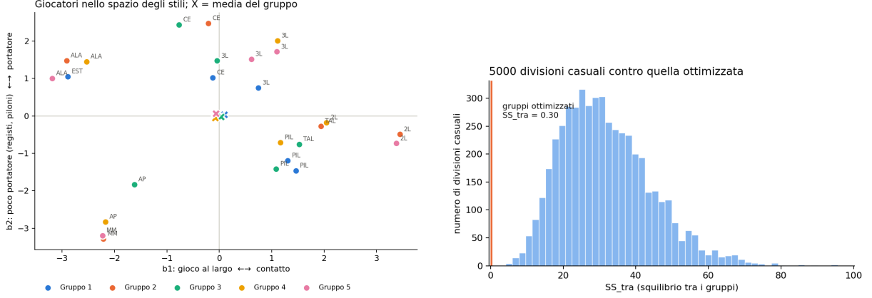
Figure 4: Left: players in the (\mathbf{b}_1, \mathbf{b}_2) plane coloured by group; the X marks are the group means, all close to the origin. Right: SS_{\text{between}} of 5000 random splits against the optimised split.
