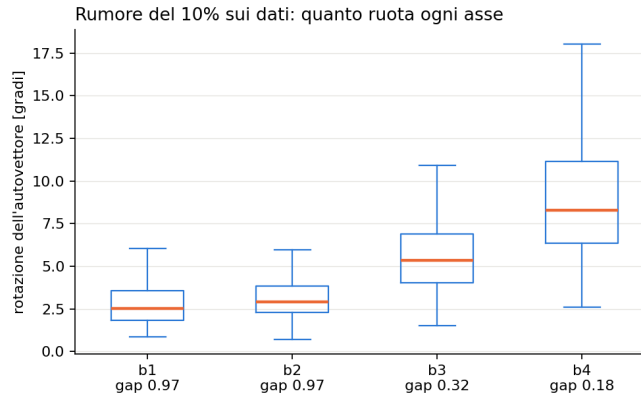
Figure 2: Rotation of the eigenvectors with 10% noise on the data: it grows as the gap shrinks.
