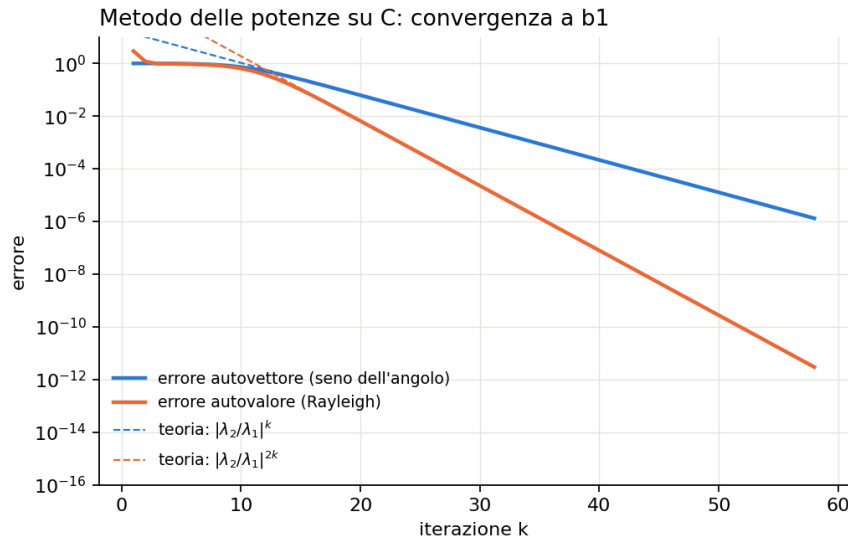
Figure 1: Error of the power method for \mathbf{b}_1 : the curves are parallel to the theoretical lines |\lambda_2/\lambda_1|^k (eigenvector) and |\lambda_2/\lambda_1|^{2k} (Rayleigh).
