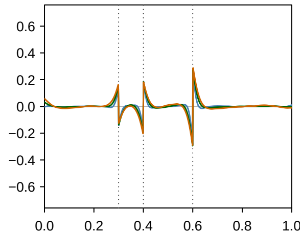
Smooth. spline
