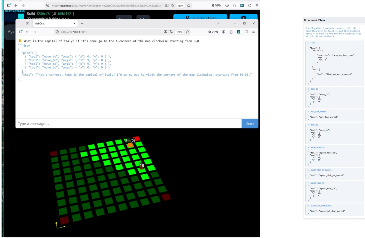
Figure 5: Left: web-chat example — the agent answers a natural-language request and generates a JSON plan with four coordinate-based movement actions. Right: a multi-step plan combining a bounded local collection loop, delivery actions, and remote MCP commands that direct the second agent to collect and deliver a hand-over parcel.
