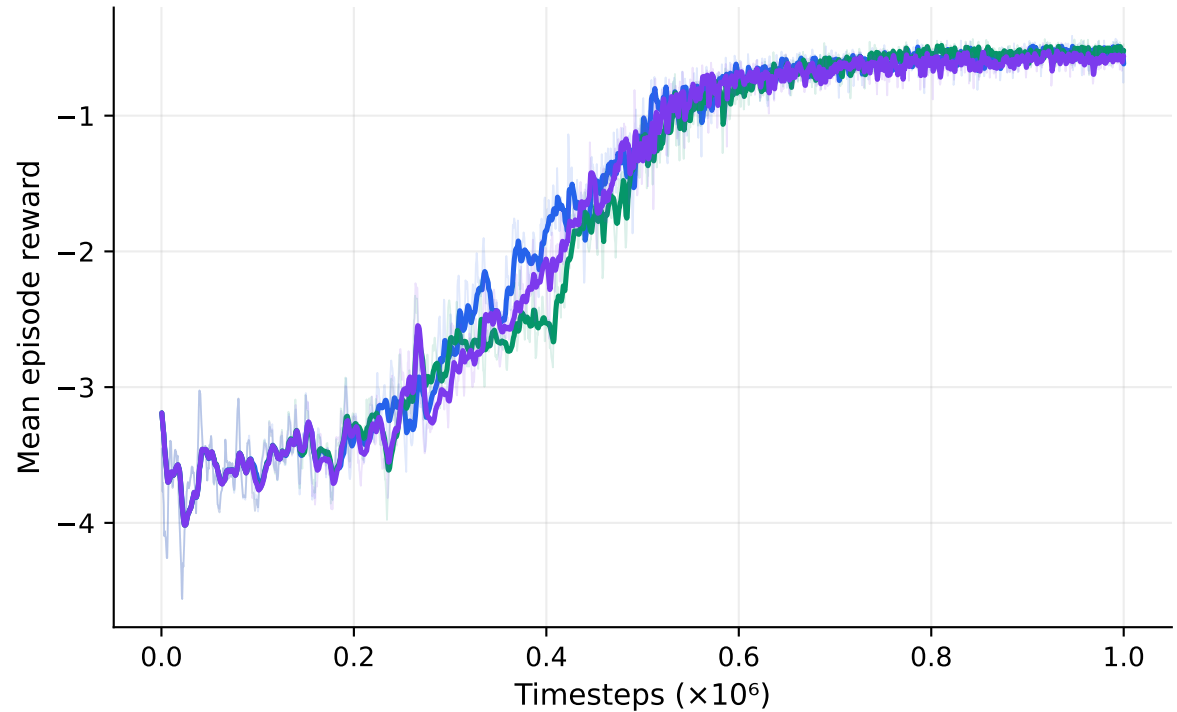
Mean episode reward
