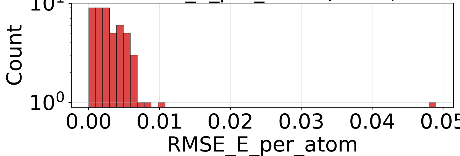
RMSE_E_per_atom (n=50)
