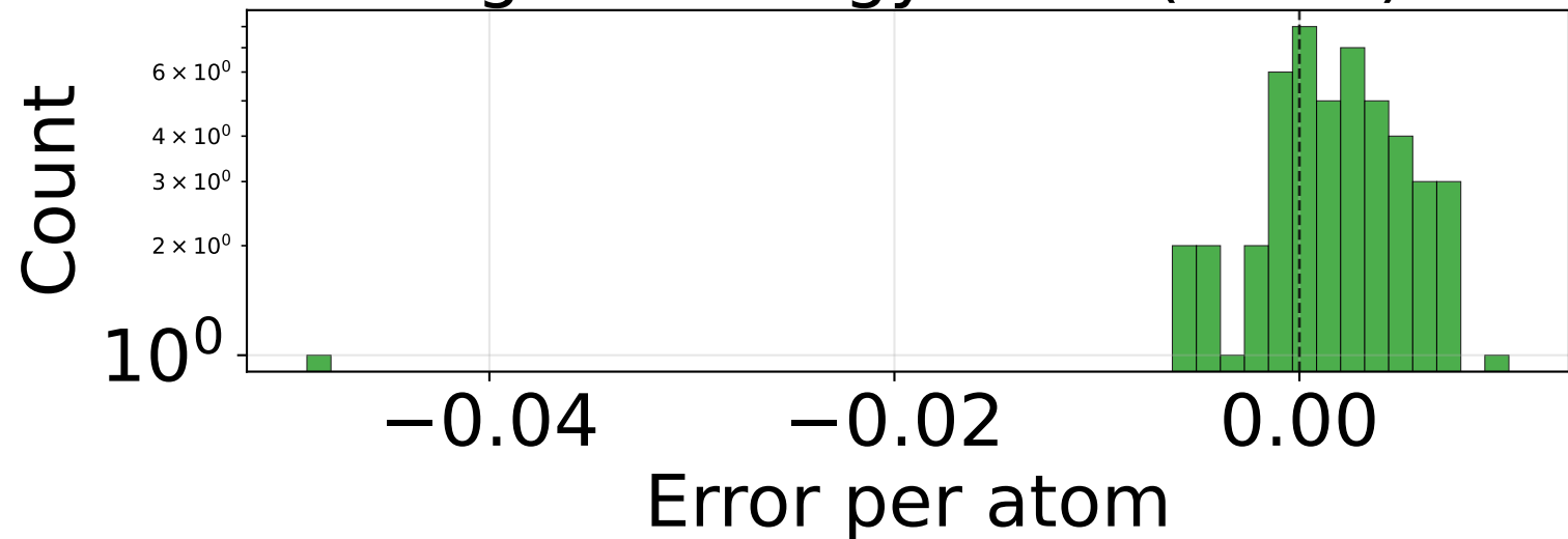
RMSE_E_per_atom (n=50)
