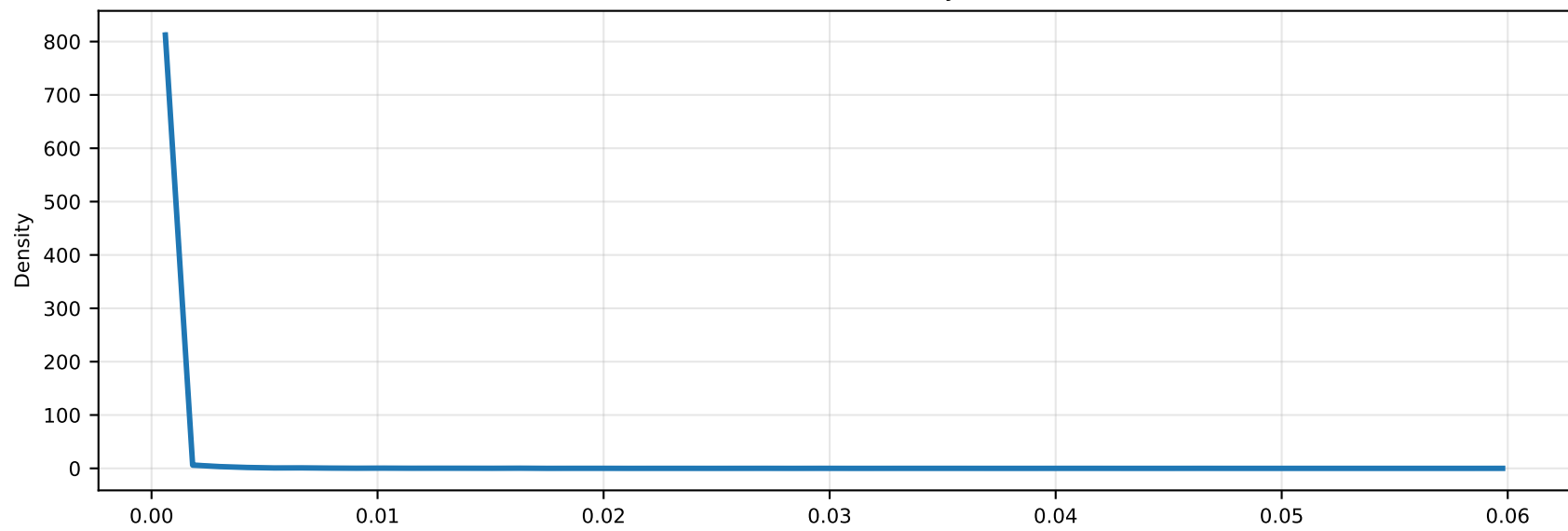
Epistemic uncertainty
