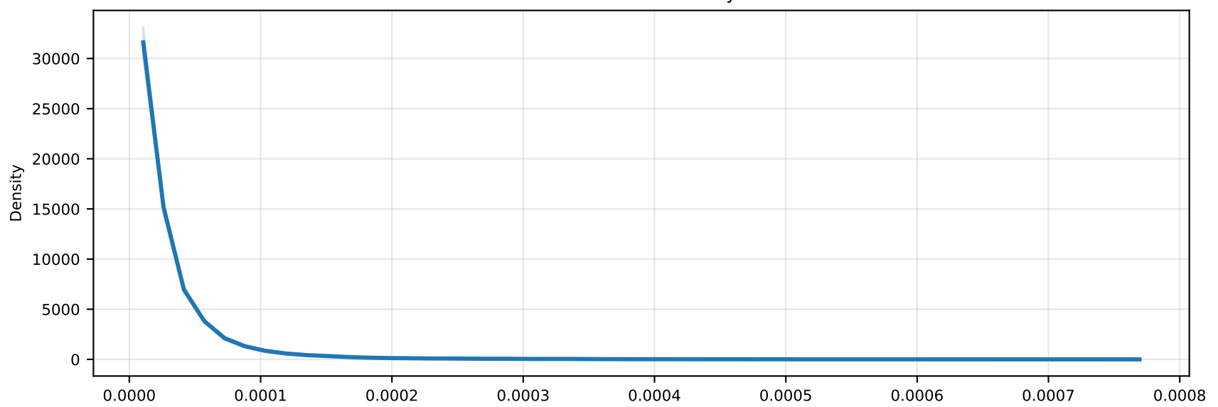
Epistemic uncertainty
