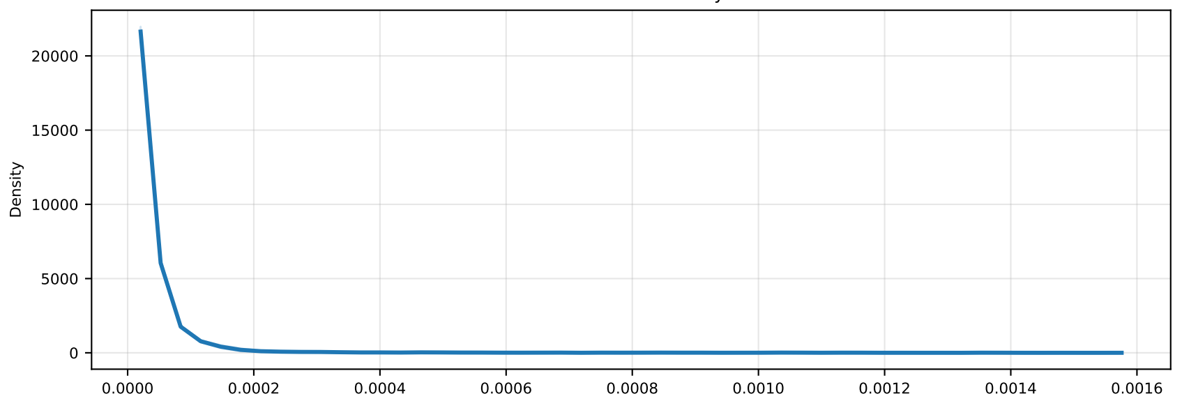
Epistemic uncertainty
