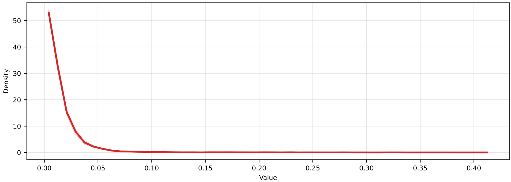
Absolute energy error
