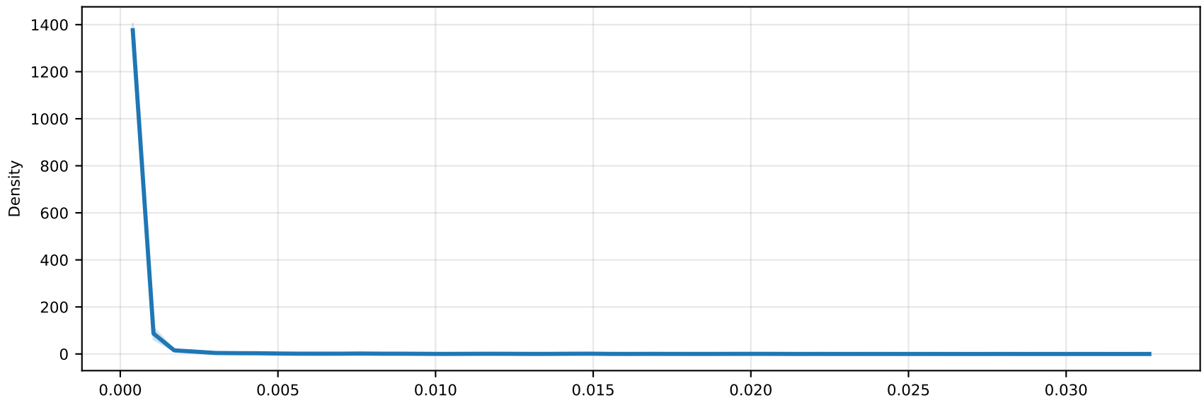
Epistemic uncertainty
