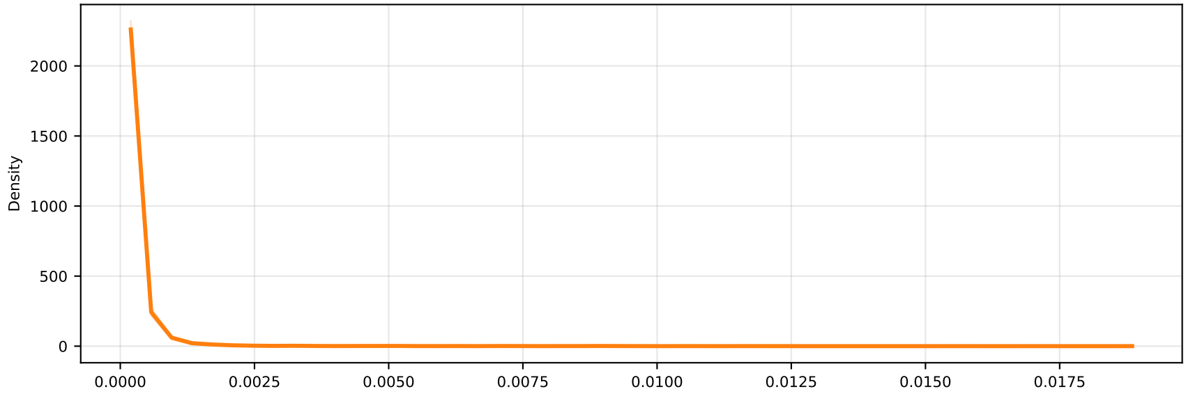
Signed energy error
