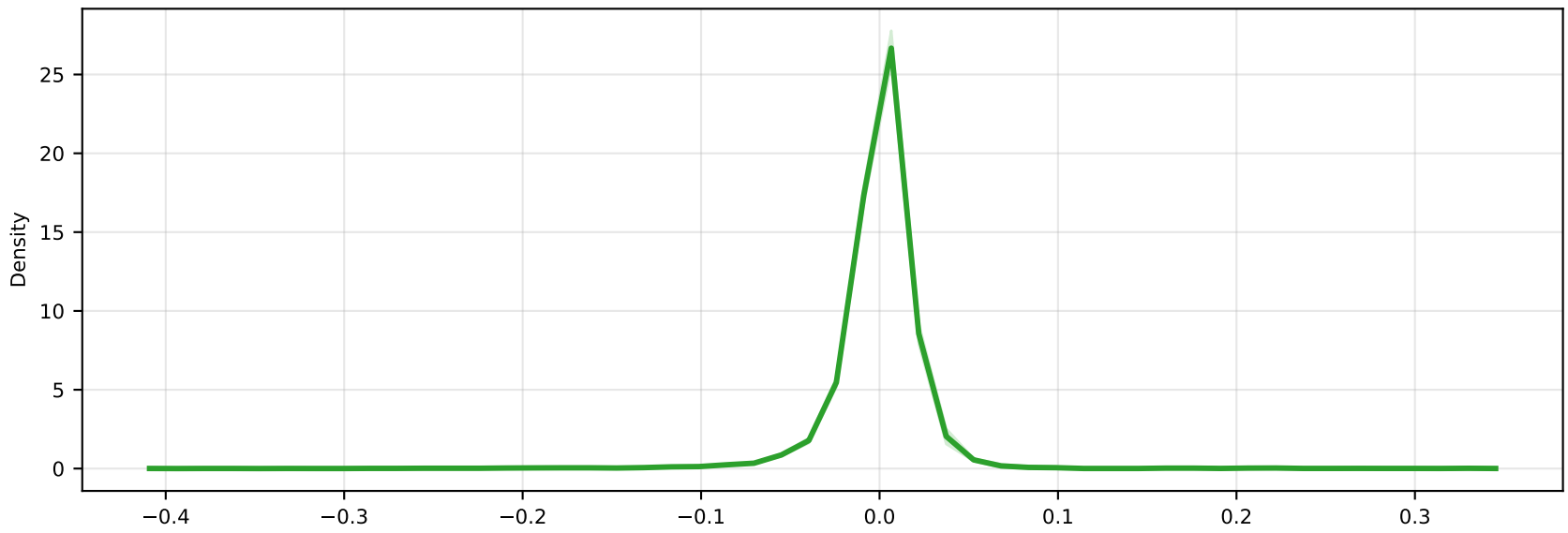
Absolute energy error
