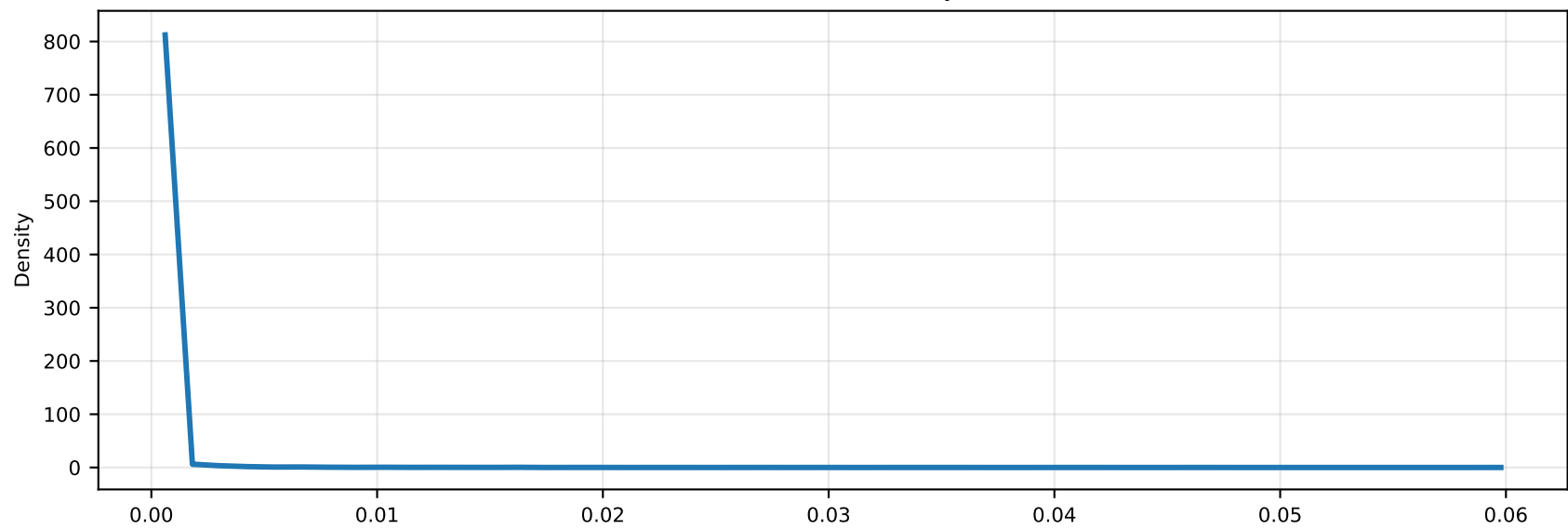
Epistemic uncertainty
