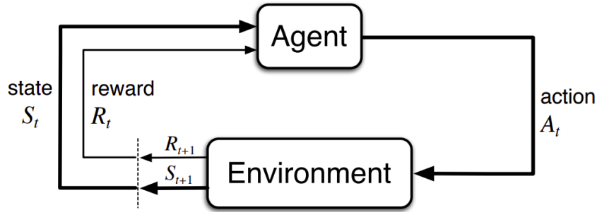
Figure 2.1. Interaction between the agent and the environment in an MDP [8].
