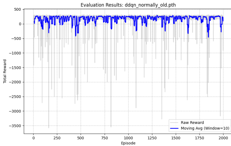
Figure 12: DDQN old standard evaluation.
