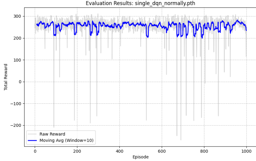
Figure 16: Single_DQN standard evaluation.
