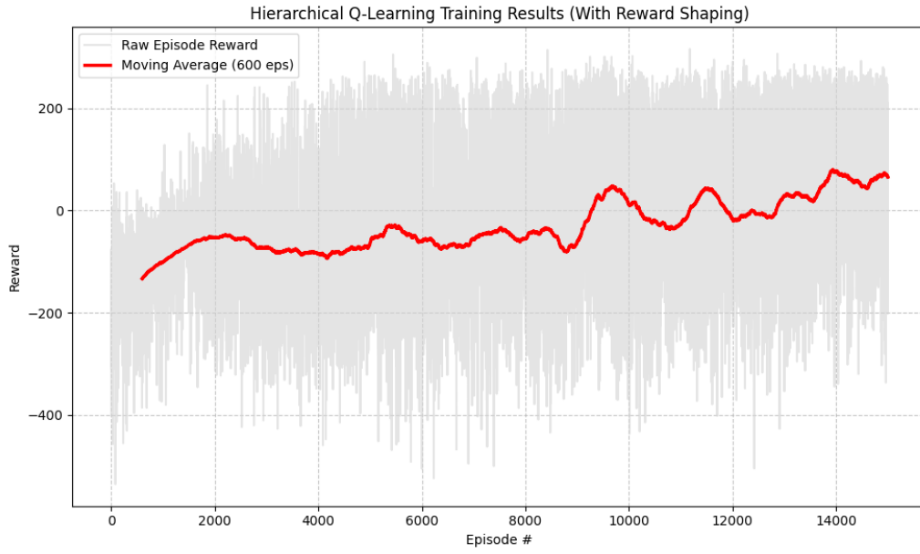
Figure 9: Tabular training with shaping.
