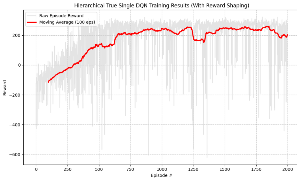
Figure 7: Single_DQN training with shaping extended.
