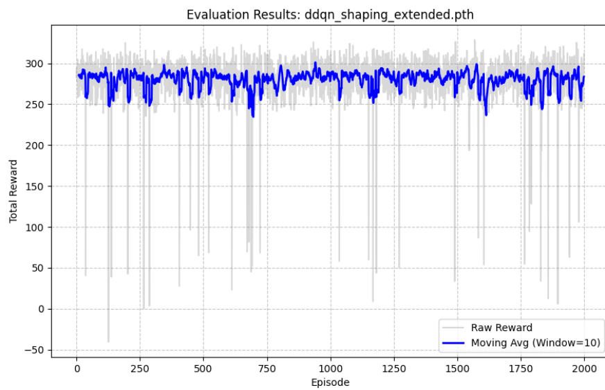
Figure 14: DDQN evaluation with shaping extended.
