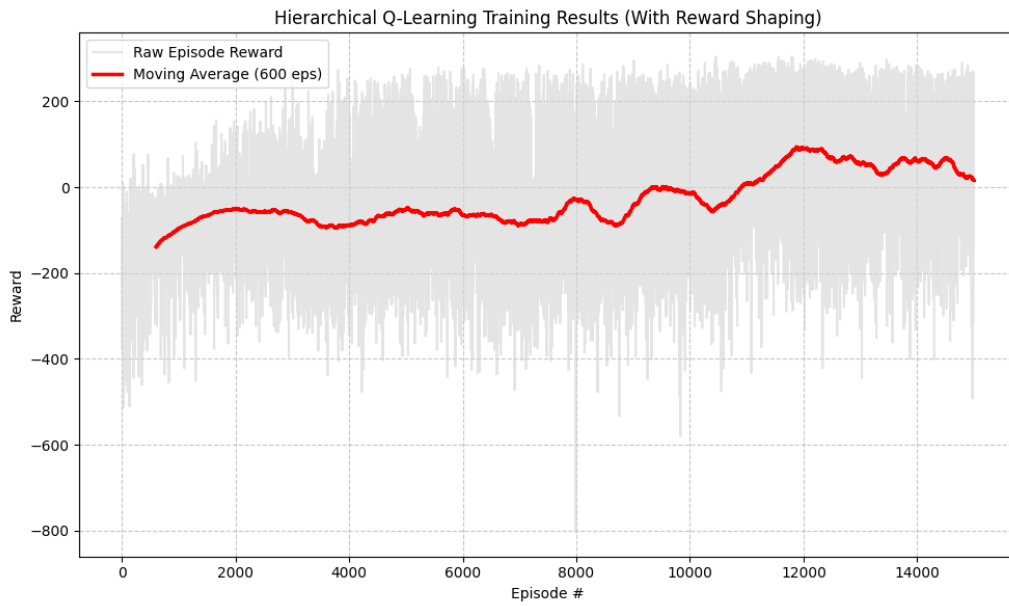
Figure 10: Tabular training with shaping extended.
