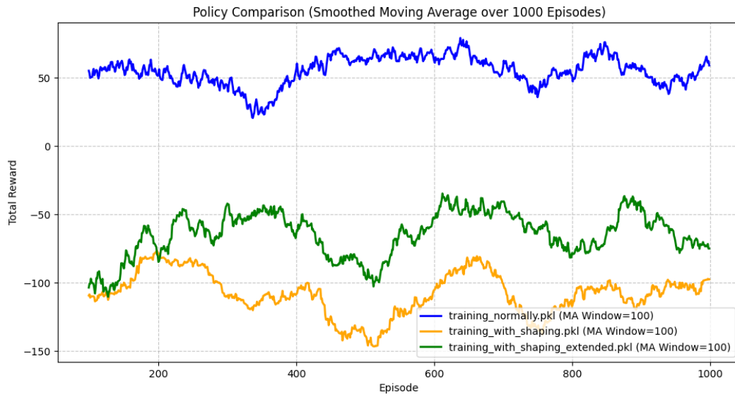
Figure 23: Tabular combined policy comparison.
