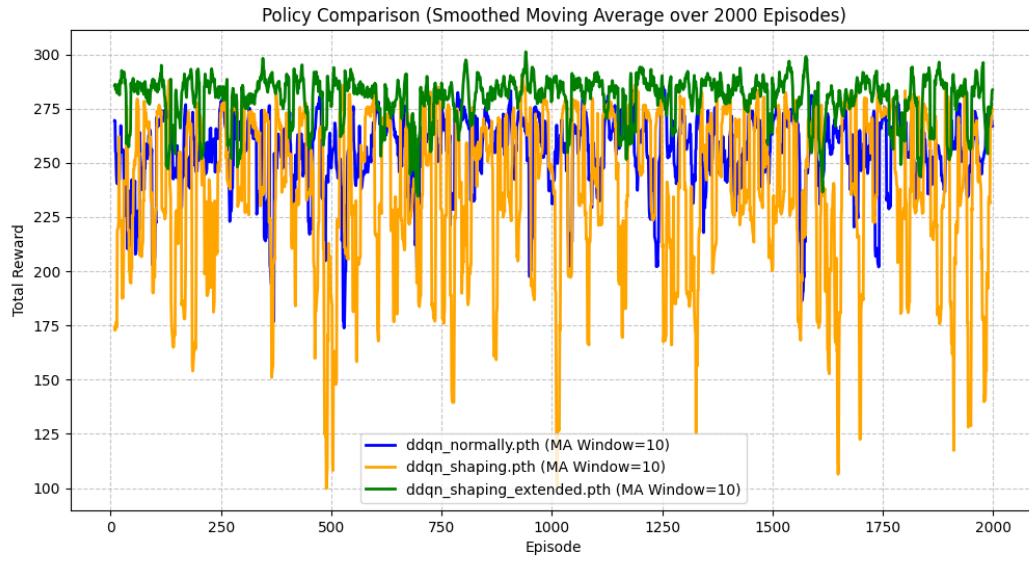
Figure 15: DDQN combined policy comparison.
