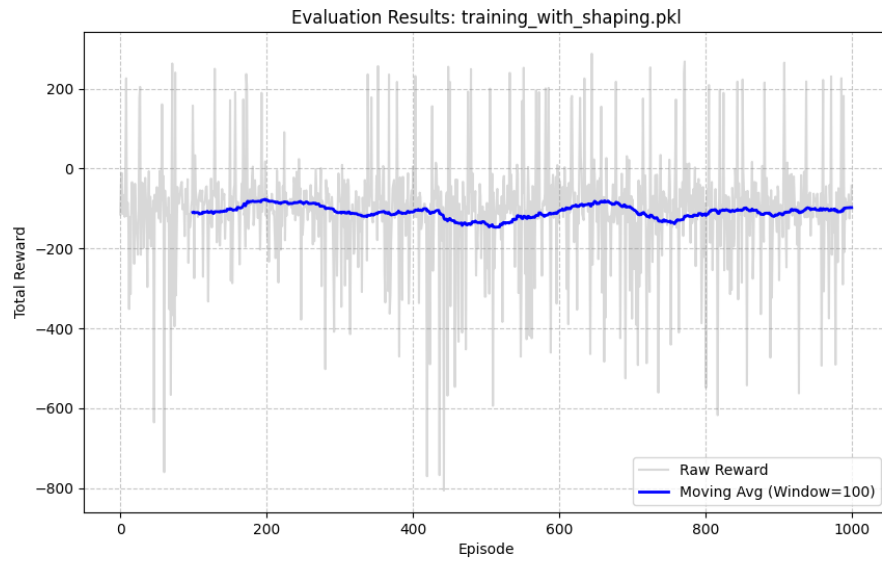
Figure 21: Tabular evaluation with shaping.
