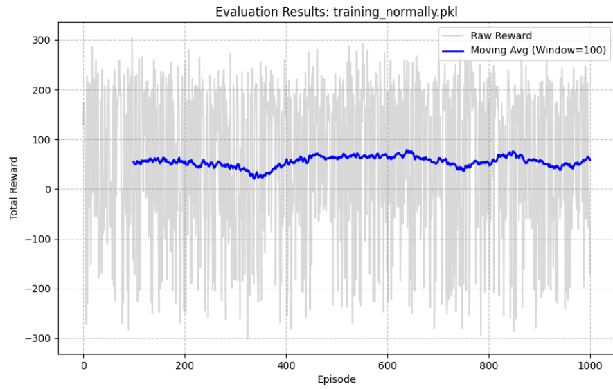
Figure 20: Tabular standard evaluation.
