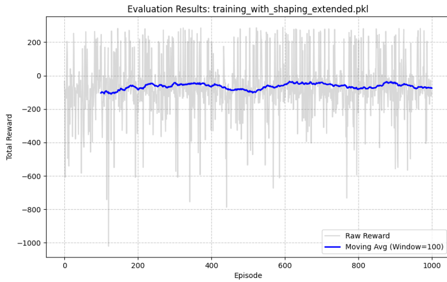
Figure 22: Tabular evaluation with shaping extended.
