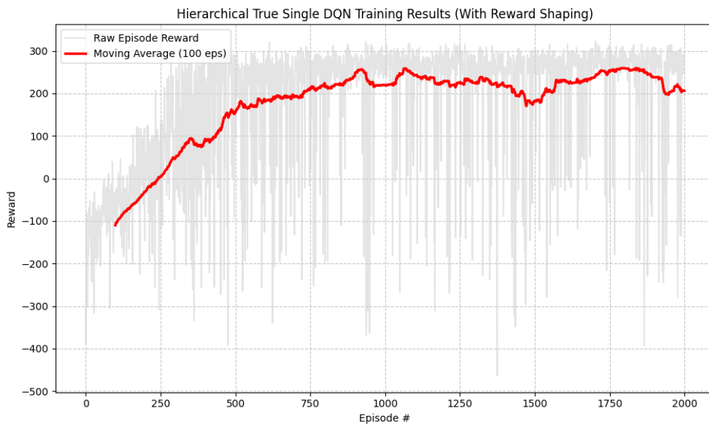
Figure 6: Single_DQN training with shaping.
