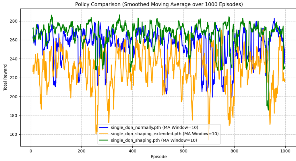
Figure 19: Single_DQN combined policy comparison.
