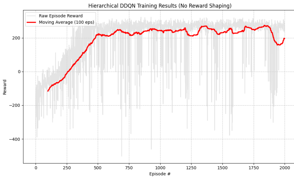
Figure 1: DDQN standard training.
