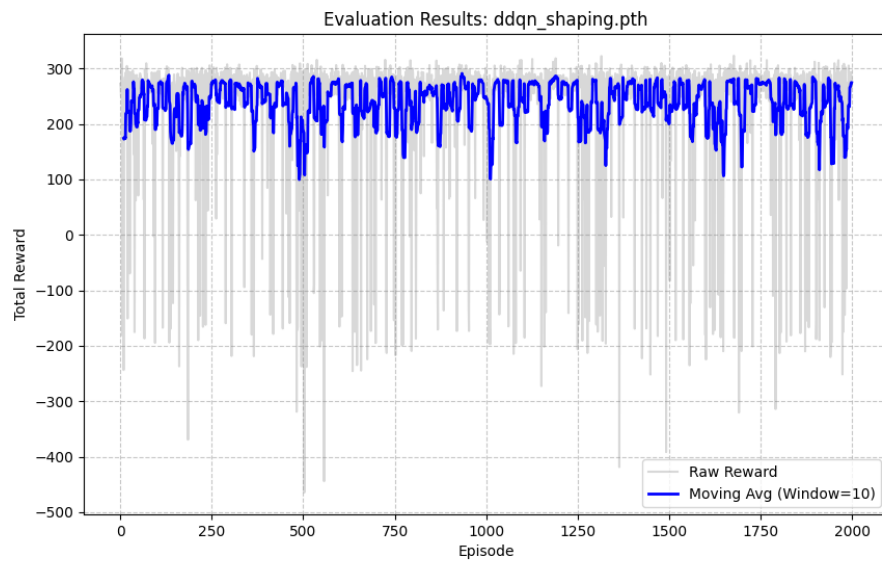
Figure 13: DDQN evaluation with shaping.
