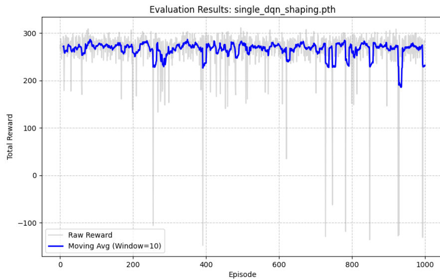
Figure 17: Single_DQN evaluation with shaping.
