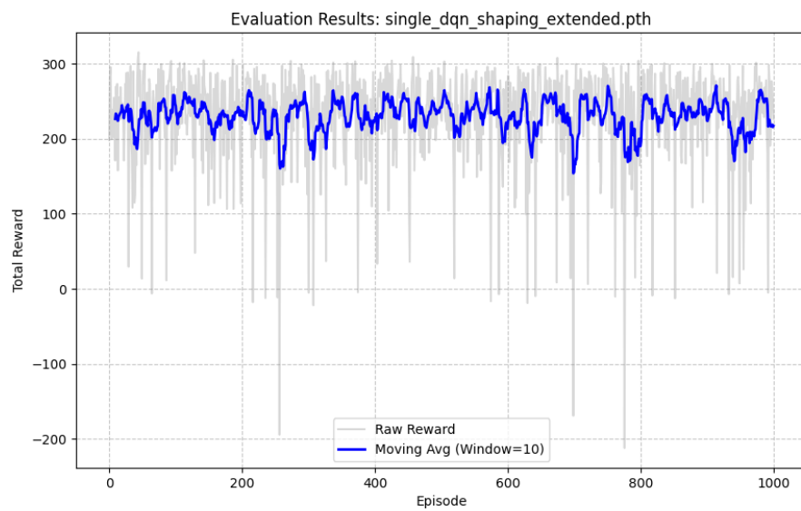
Figure 18: Single_DQN evaluation with shaping extended.
