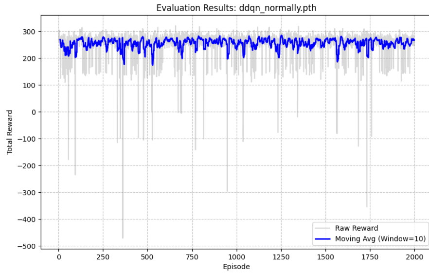
Figure 11: DDQN standard evaluation.
