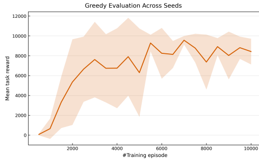
Figure 4.7. 1-phase task. Periodically greedy evaluation of the standalone unbiased policy.
