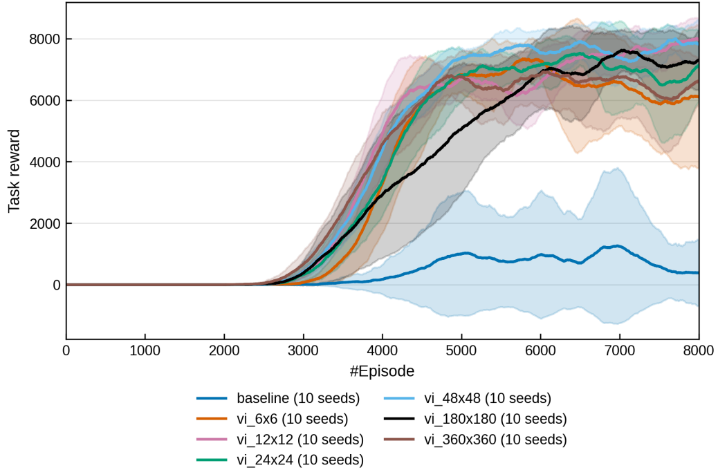
Figure 4.13. 2-phase trajectory. Training task reward for the baseline and the six abstraction grid resolutions, using ten seeds per configuration.
