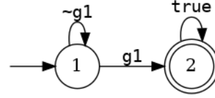
Figure 4.4. DFA for the 1-phase task.
