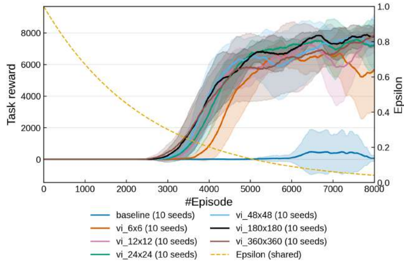
Figure 4.19. 3-phase trajectory – Simple. Training task reward for the baseline and the six abstraction grid resolutions, using ten seeds per configuration.
