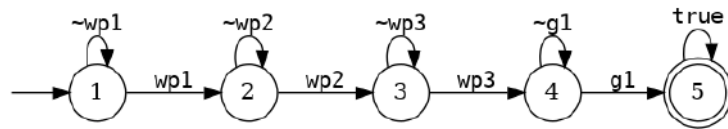
Figure 4.25. DFA for the 4-phase task.
