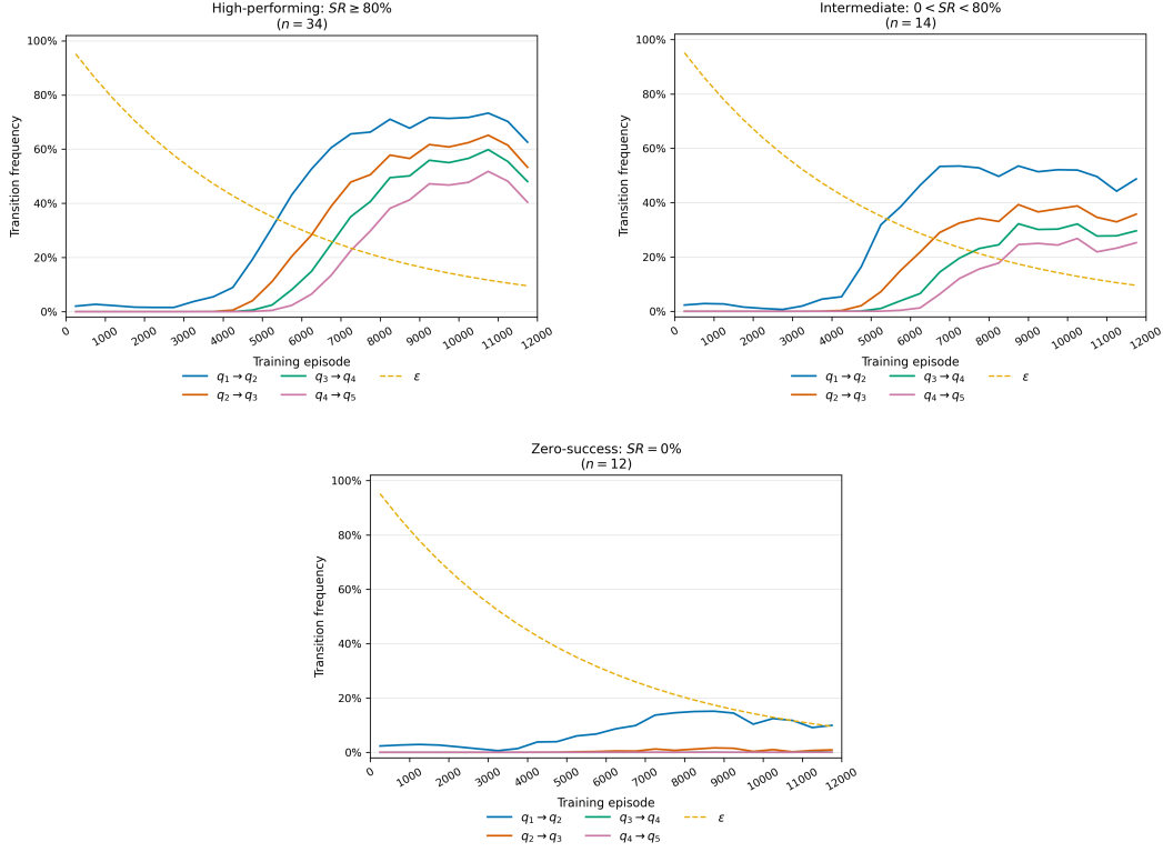
Figure 4.30. 4-phase trajectory. DFA-transition frequencies during training, grouped by the post-training success rate of the best policy: high-performing ( SR \geq 80\% ), intermediate ( 0 < SR < 80\% ), and zero-success ( SR = 0\% ) runs. Each curve reports the fraction of episodes containing the corresponding transition, computed over non-overlapping windows of 500 episodes and averaged across the runs in each group.
