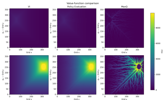
Value functions for VI, policy evaluation, and MaxQ (top: q_1 ; bottom: q_2 ).
