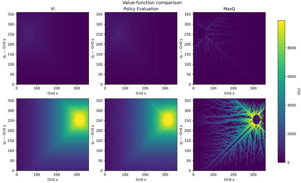
Figure 4.38. 2-phase trajectory. Comparison of value functions on the 360 \times 360 abstract grid. Columns show, from left to right, the Value Iteration reference, the value function obtained through Policy Evaluation of the learned unbiased greedy policy, and the direct estimate \max_a Q(s, a) . The top and bottom rows correspond to DFA states q_1 and q_2 , respectively.
