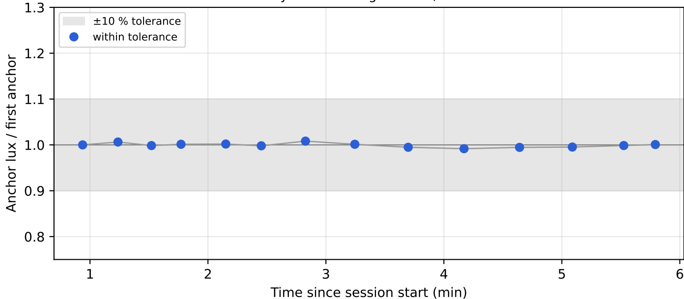
Anchor stability: B255 at brightness 8, reference 30.3 lx
