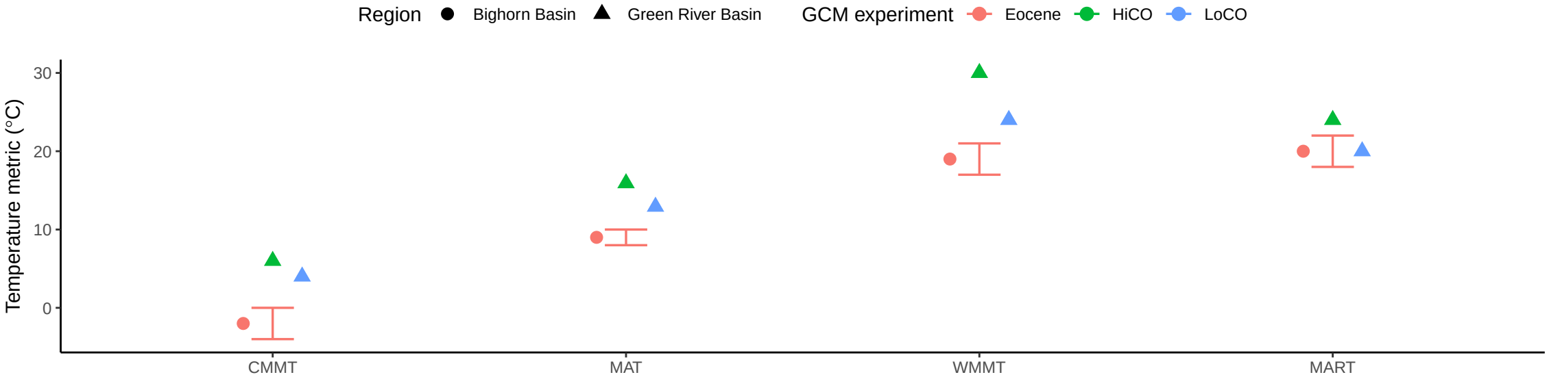
Regional Eocene GCM benchmarks Equilibrium climate states; points are not assigned to proxy ages
