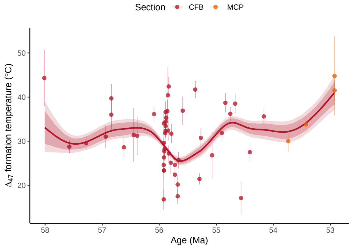
BHB soil-carbonate formation temperature Age-binned CFB and MCP Delta47; no extrapolation beyond observations
