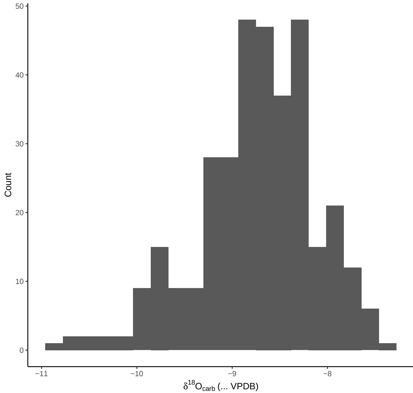
Retained Bowen \delta^{18}\text{O}_{\text{carb}} Values
