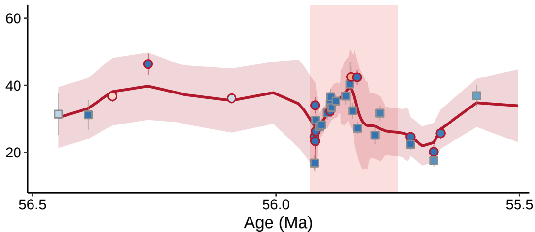
C CFB \delta^{18}\text{O}_{\text{water}}
