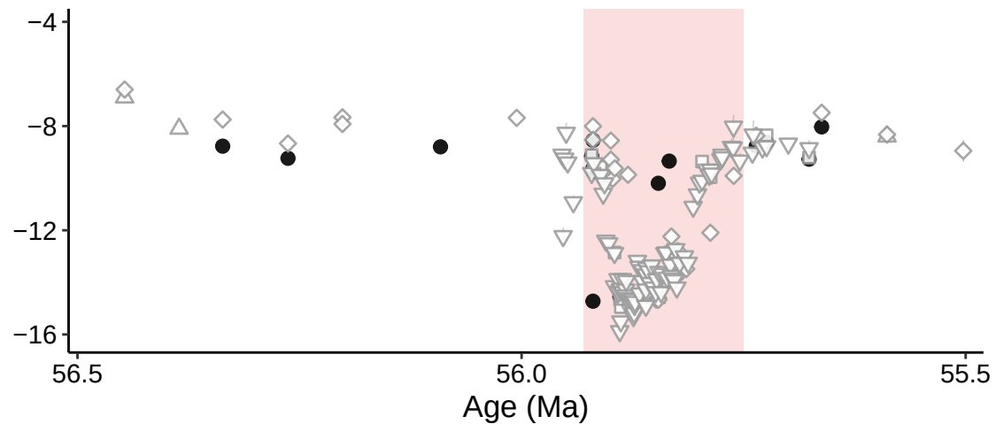
D CFB \Delta^{17}\text{O}_{\text{water}}
