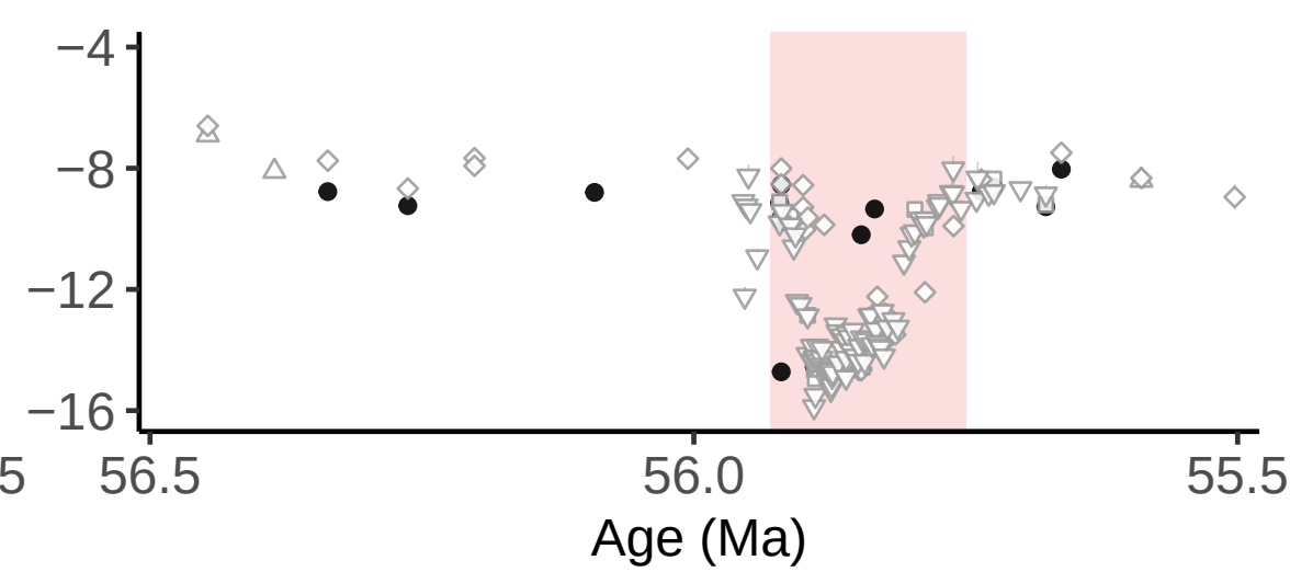
D CFB \Delta^{17}\text{O}_{\text{water}}
