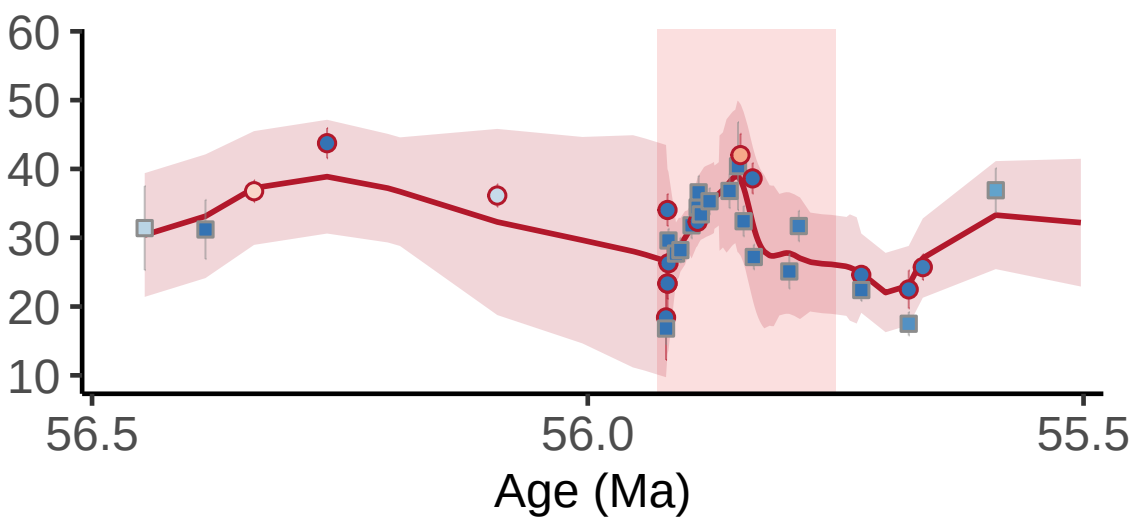
C CFB \delta^{18}\text{O}_{\text{water}}
