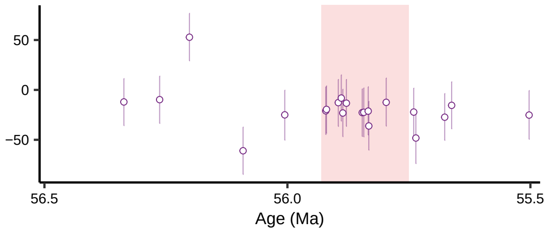
D CFB \Delta^{17}\text{O}_{\text{water}}
