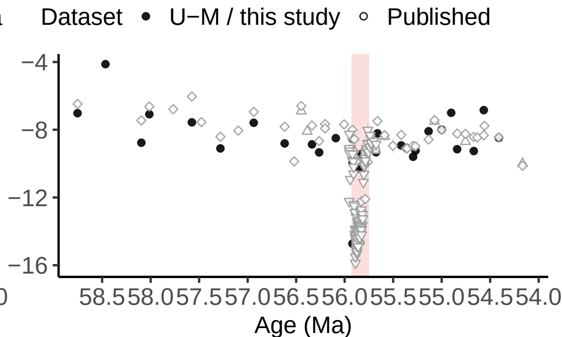
D CFB \Delta^{17}\text{O}_{\text{water}}
