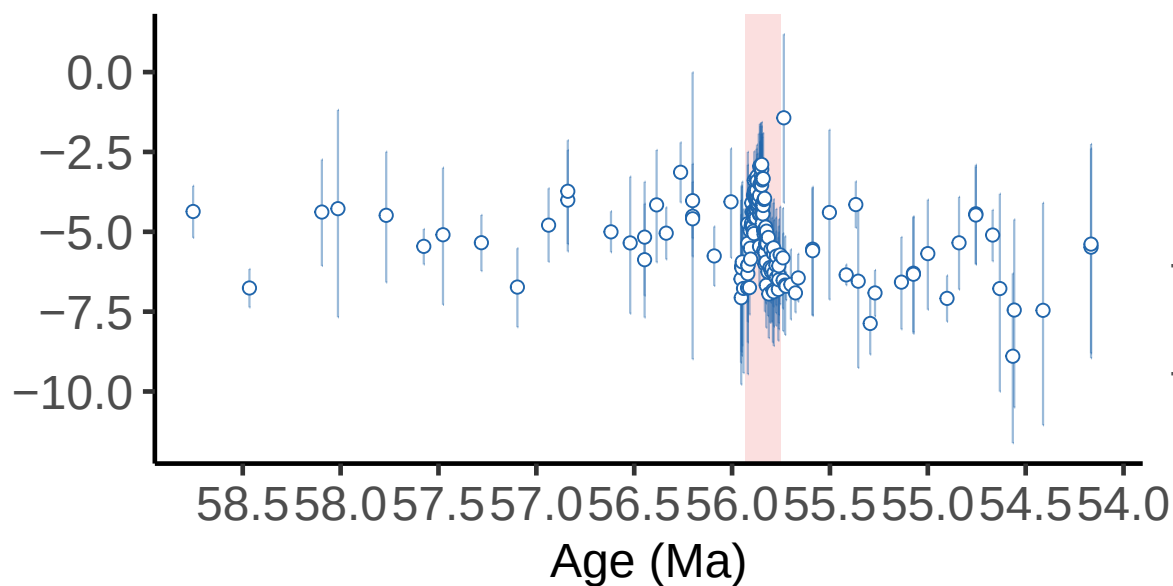
C CFB \delta^{18}\text{O}_{\text{water}}
