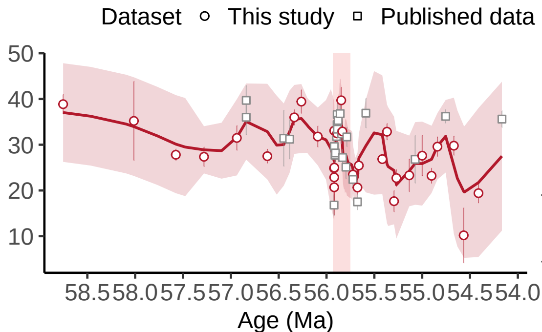
C CFB \delta^{18}\text{O}_{\text{water}}
