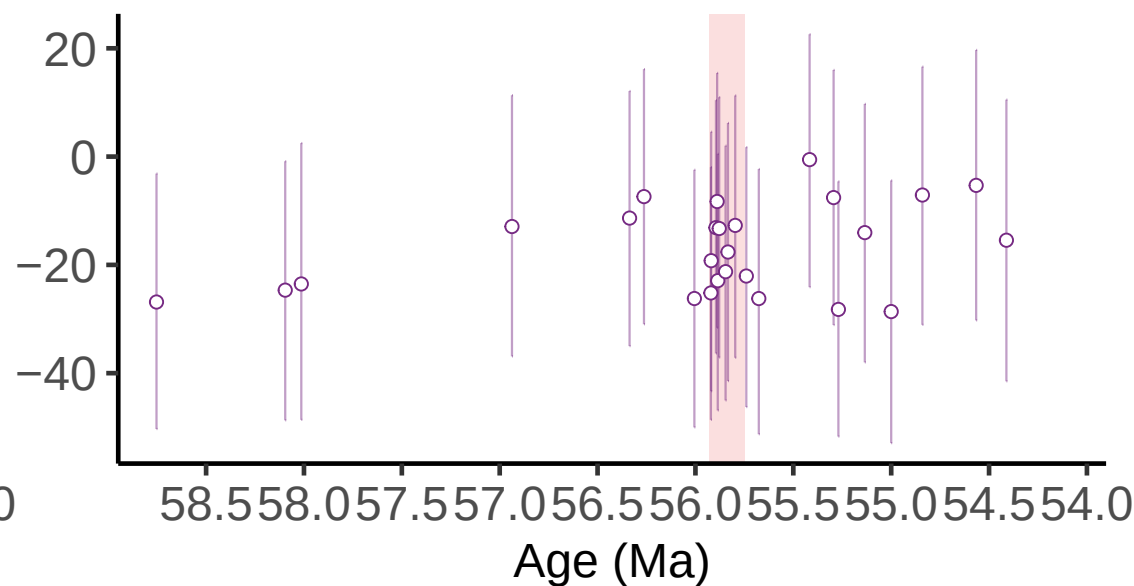
D CFB \Delta^{17}\text{O}_{\text{water}}
