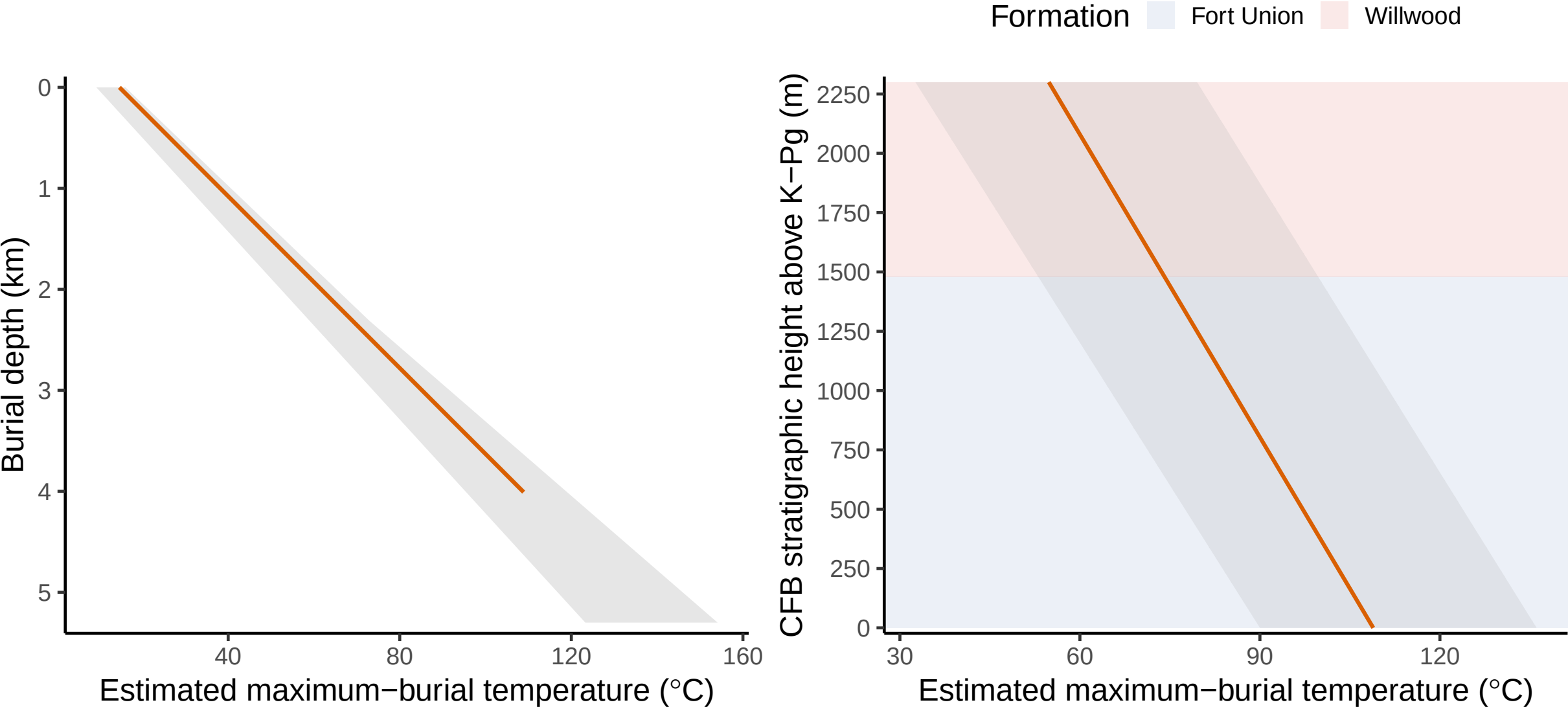
A Roberts et al. (2008) burial-temperature scenario Orange = McCulloch Peak; grey = full BHB model range B Thermal projection through the CFB corridor Orange = McCulloch Peak; grey = full Roberts et al.
