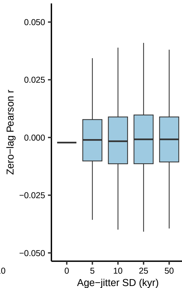
Age-jitter sensitivity
