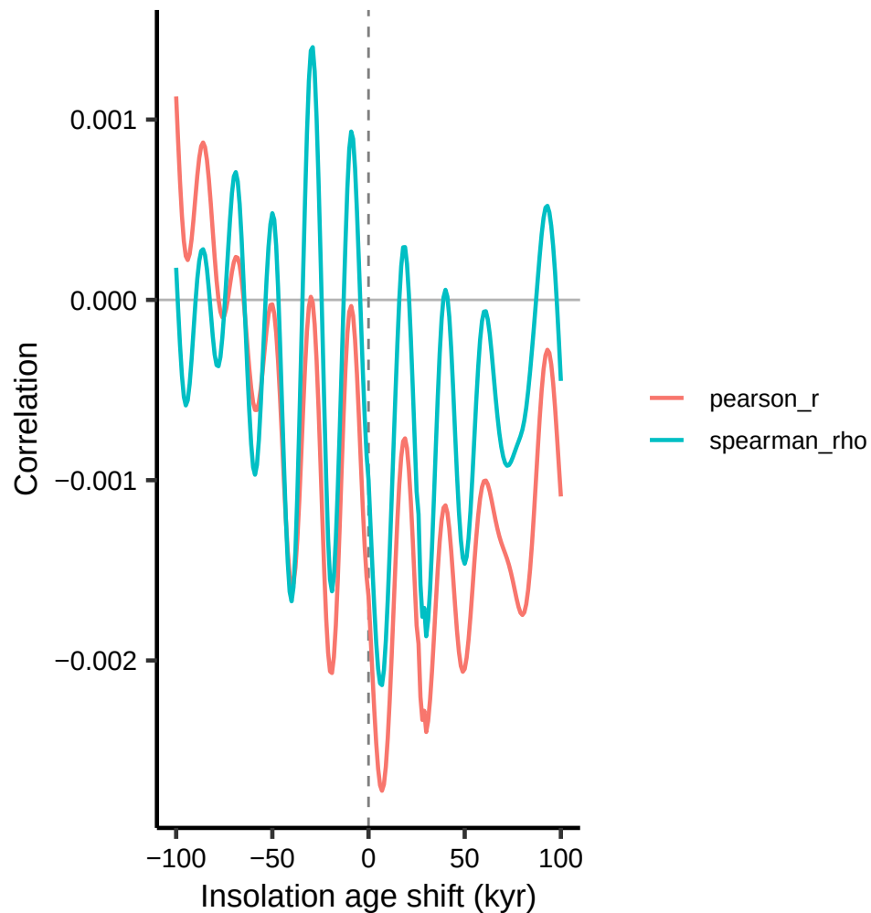
Lag sensitivity
