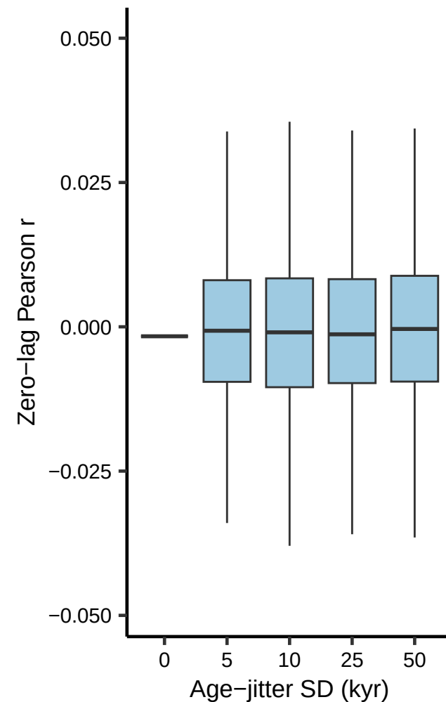
Age-jitter sensitivity
