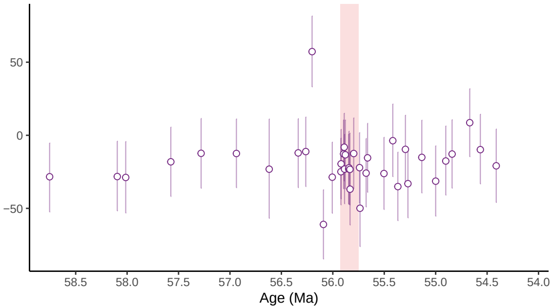
D CFB \Delta^{17}\text{O}_{\text{water}}
