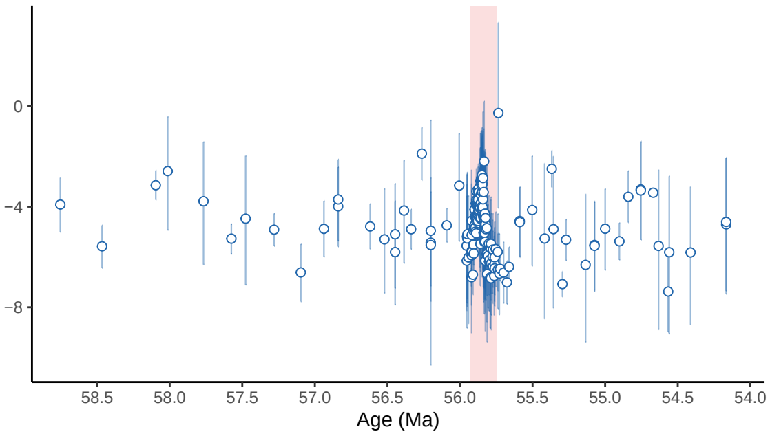
C CFB \delta^{18}\text{O}_{\text{water}}
