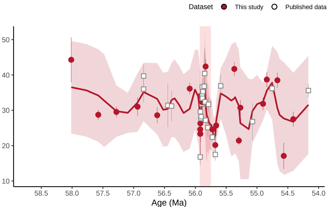
C CFB \delta^{18}\text{O}_{\text{water}}
