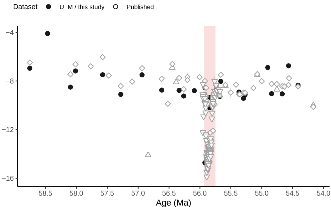
D CFB \Delta^{17}\text{O}_{\text{water}}
