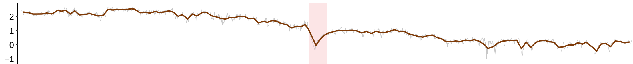
C Bighorn Basin soil–carbonate \delta^{13}\text{C} (per mil VPDB)
