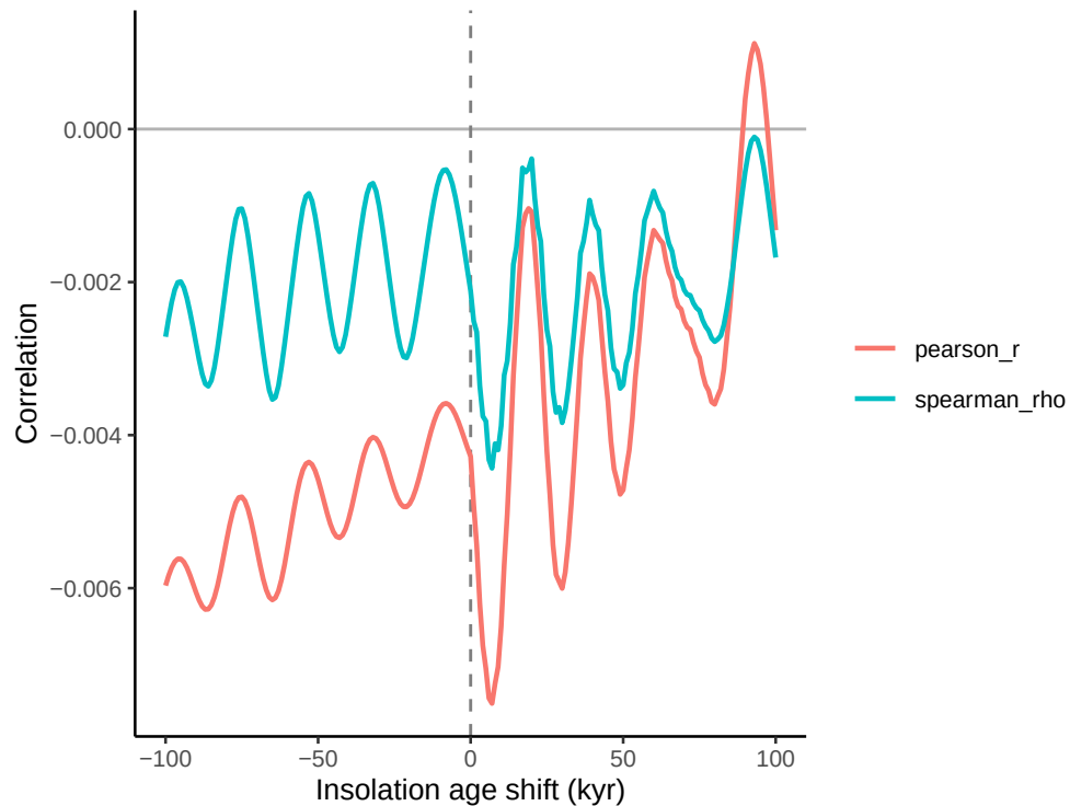
Lag sensitivity
