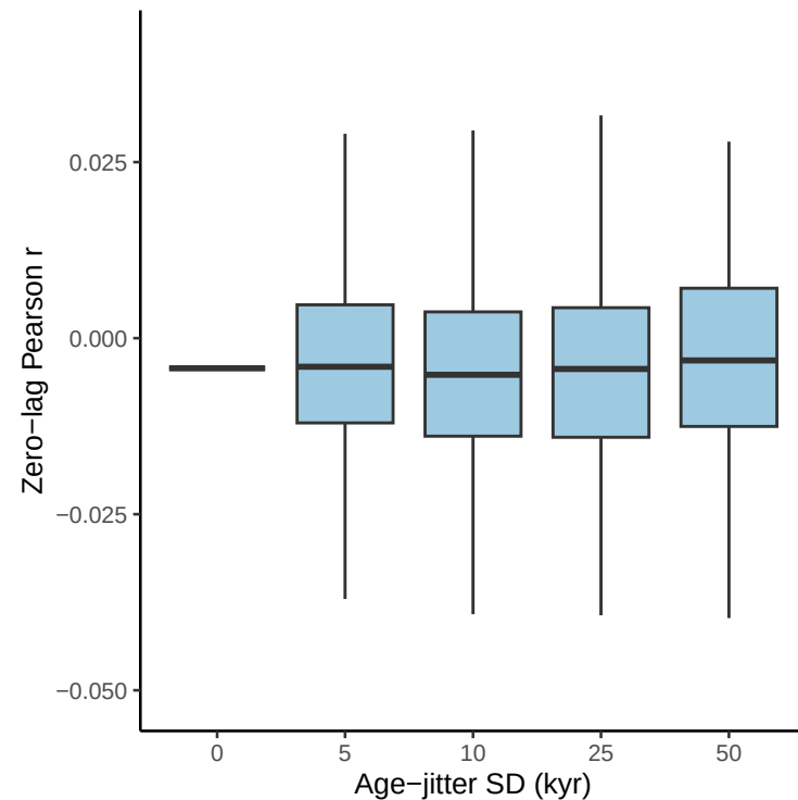
Age-jitter sensitivity
