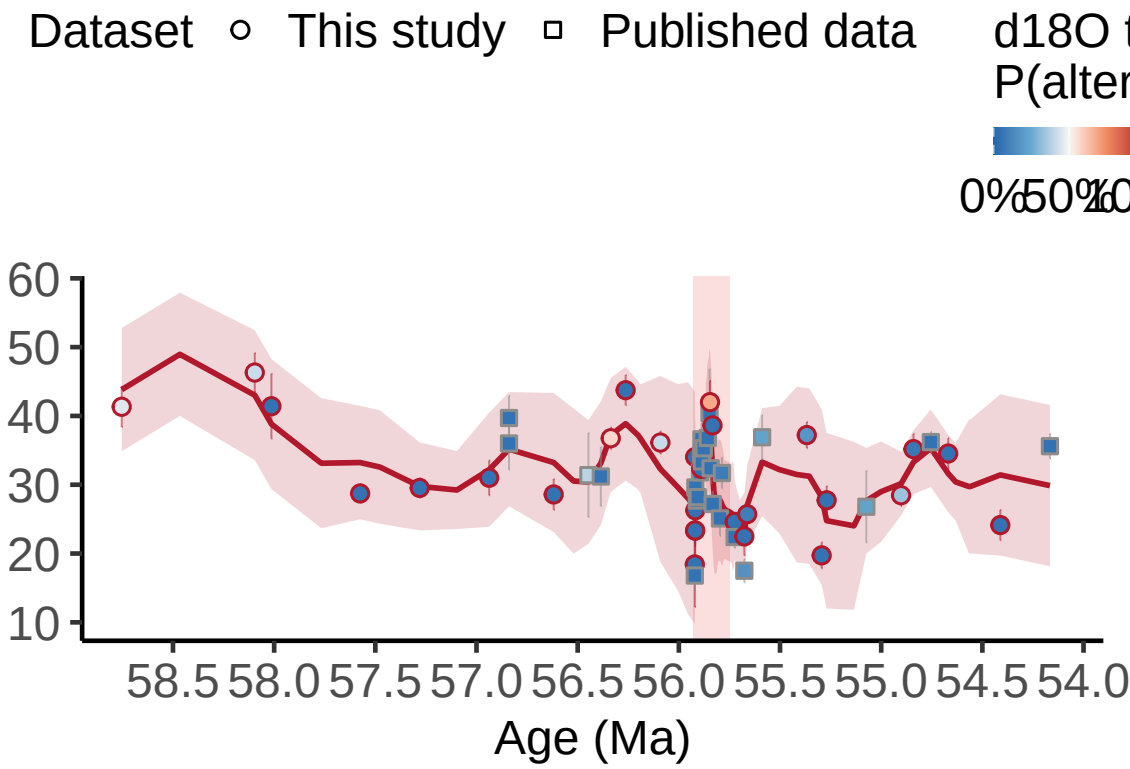
C CFB \delta^{18}\text{O}_{\text{water}}
