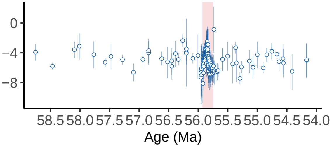
C CFB \delta^{18}\text{O}_{\text{water}}
