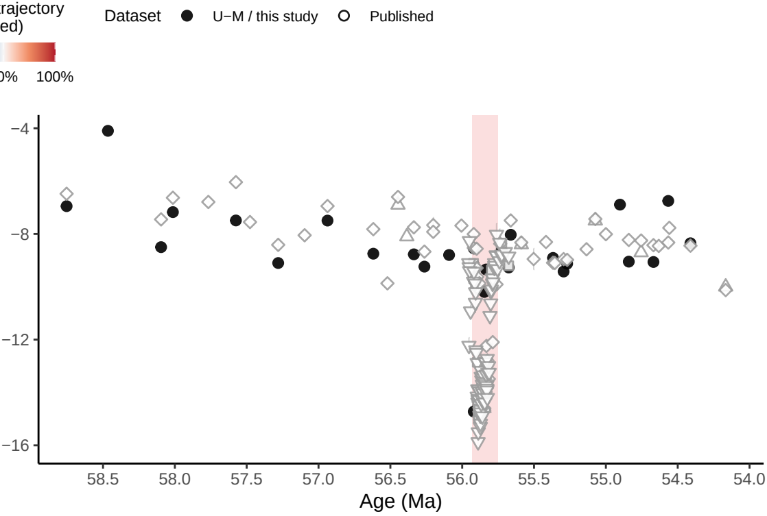
D CFB \Delta^{17}\text{O}_{\text{water}}
