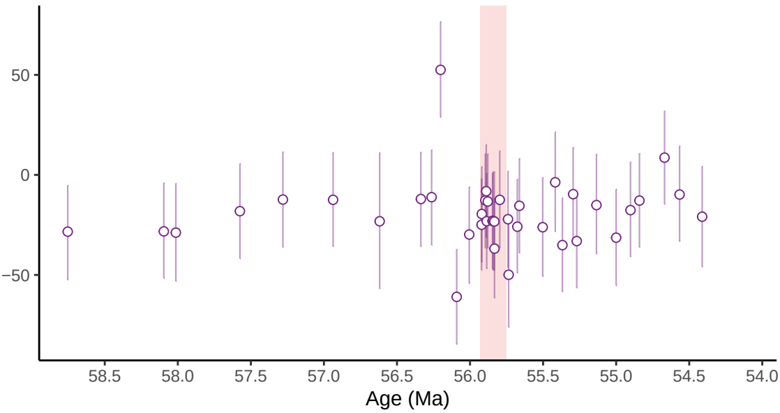
D CFB \Delta^{17}\text{O}_{\text{water}}
