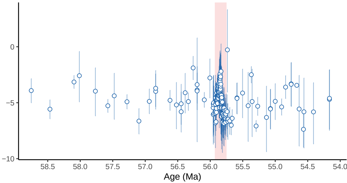
C CFB \delta^{18}\text{O}_{\text{water}}
