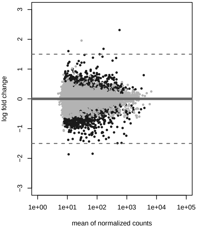
GOA_TC normal
