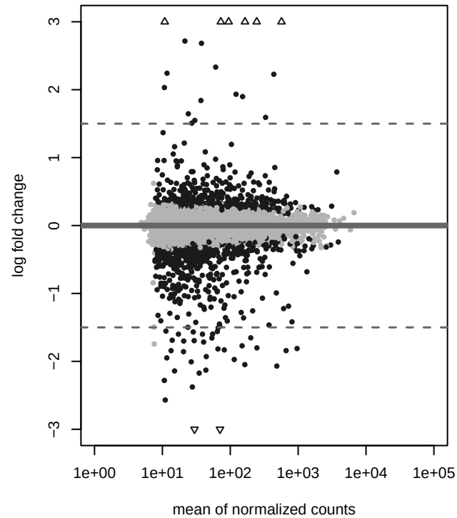
GOA_TC ashr
