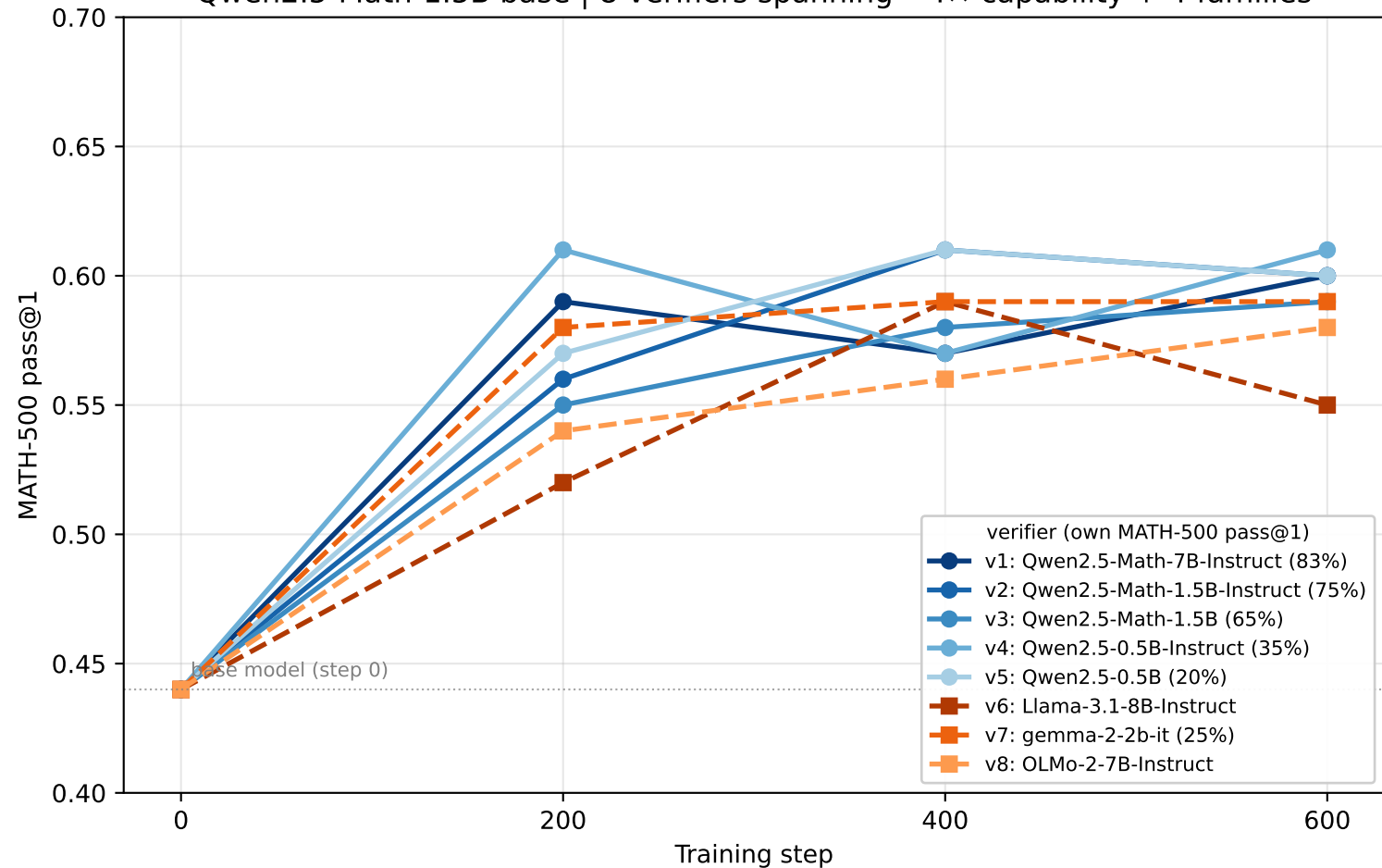
Generator MATH-500 across verifier sweep Qwen2.5-Math-1.5B base | 8 verifiers spanning \sim 4\times capability + 4 families
