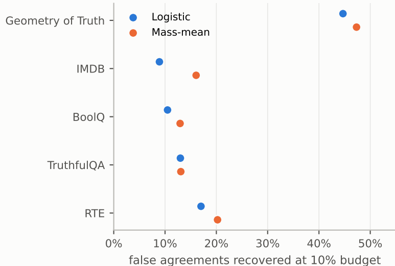
B Operating point
