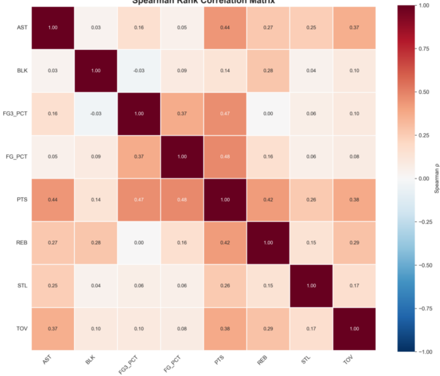
Copula Dependency Heatmap Spearman Rank Correlation Matrix
