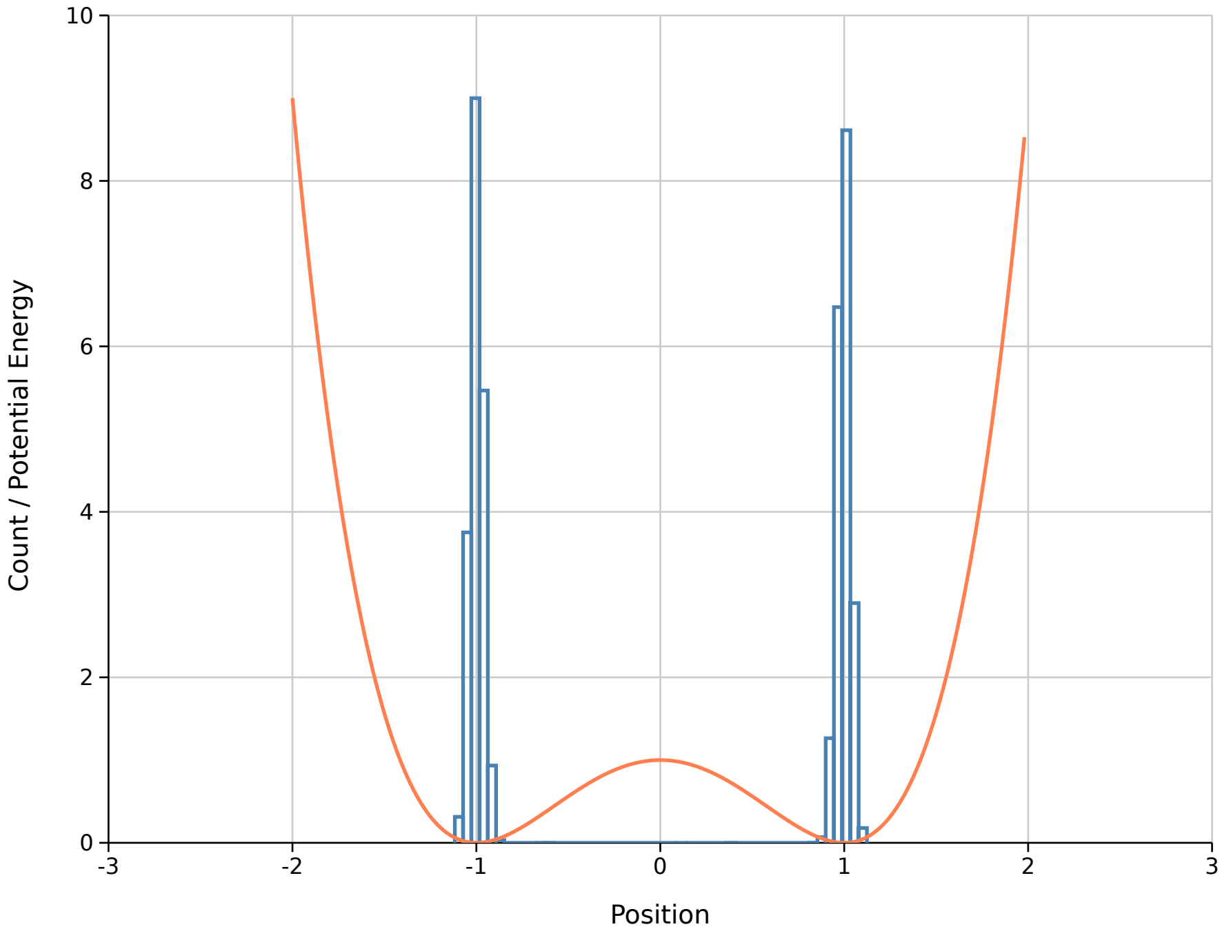
Histogram of Chain Samples with Potential Function
