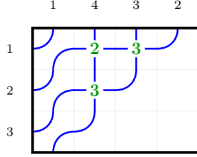
(a) The RC graph R ; the crossing (2, 2) has right root (3, 4)
