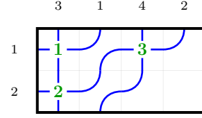
(b) \mathcal{Z}(R) , of height 2
