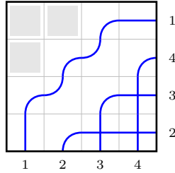
(a) \Phi(R) , w_R = 1432
