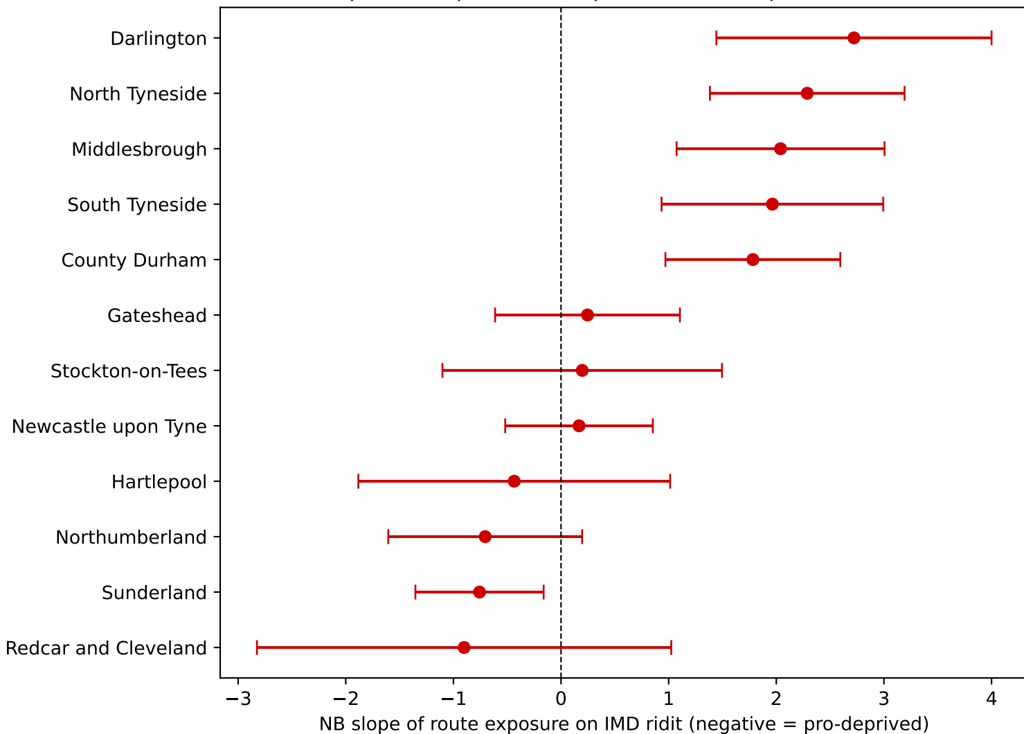
LA-specific deprivation slopes for route exposure (95% CI)
