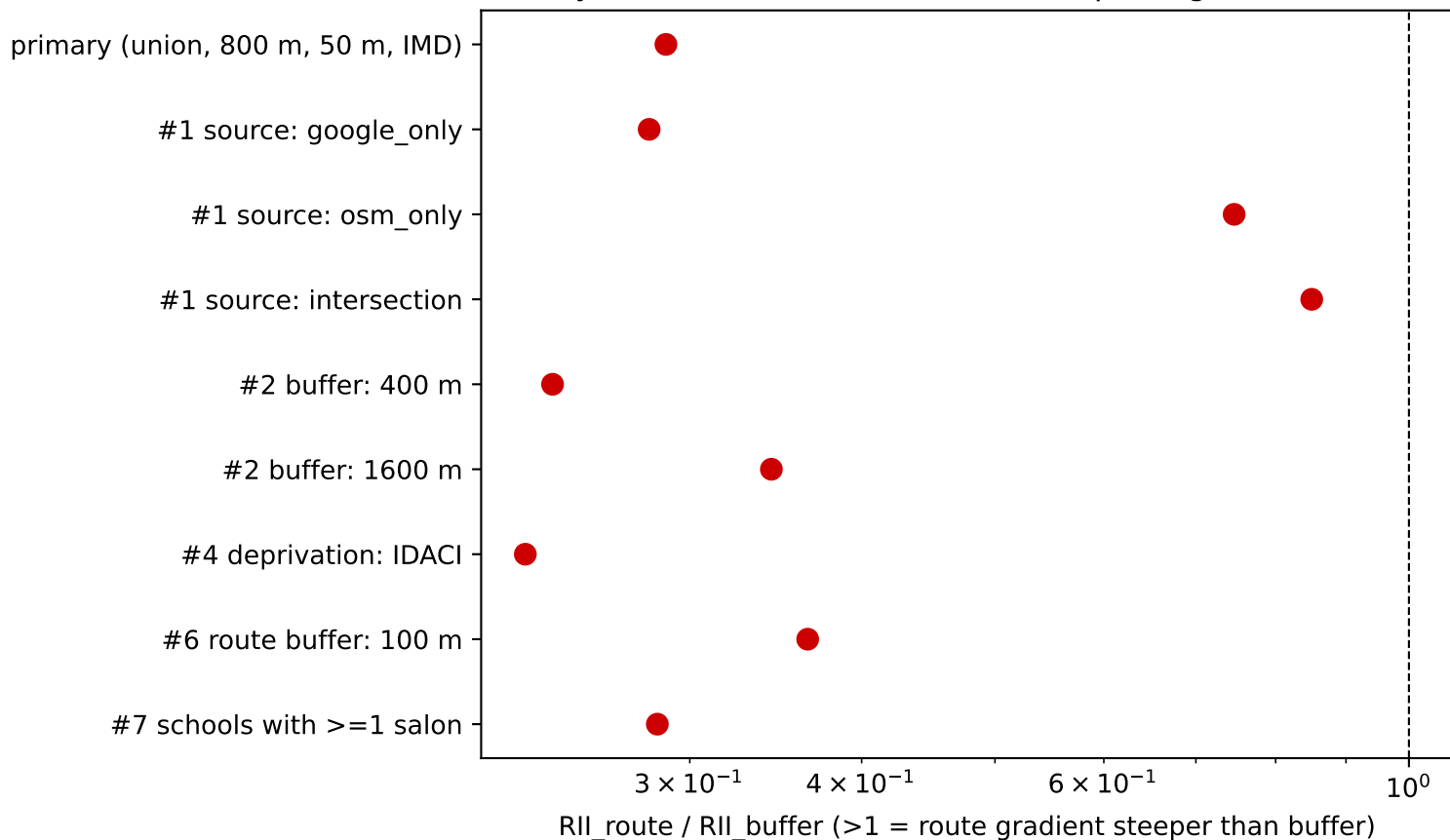
Sensitivity of the headline H2 ratio across pre-registered dimension
